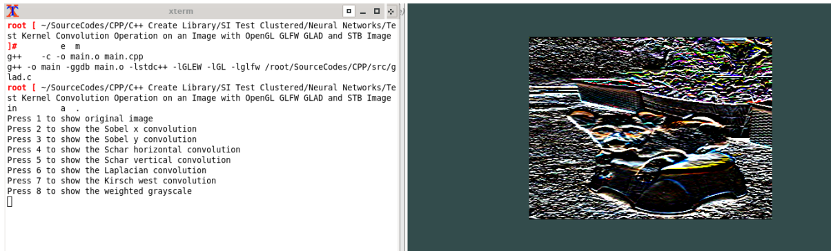
Figure 10.37: By pressing keyboard keys from 1 to 8, we can alternate and see the convoluted image ( SymIntegration/Examples/Neural Networks/Test Kernel Convolution Operation on an Image with OpenGL GLFW GLAD and STB Image/main.cpp ).
