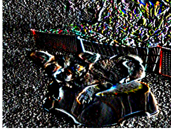
Figure 10.33: The Schar horizontal operation on an image (SymIntegration/Examples/Neural Networks/Test Kernel Convolution Operation on an Image with OpenGL GLFW GLAD and STB Image/main.cpp).
