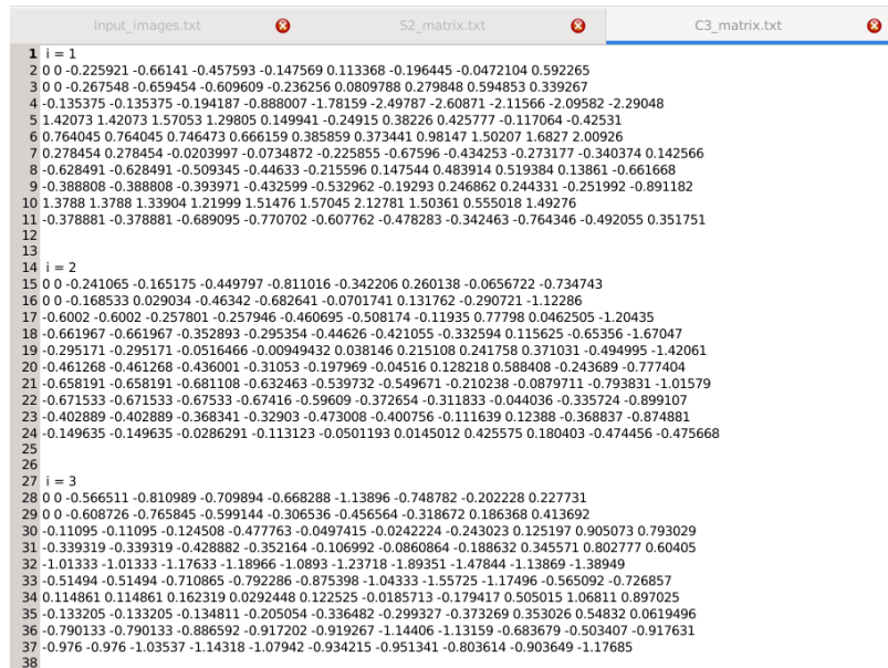
Figure 10.55: The C3 feature maps after performing convolution operation with sparse connectivity with S2 layer.
