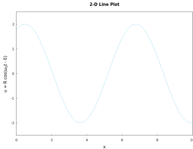
Figure 3.19: The graph of Eq. (3.157), or the equivalent Eq. (3.155), for a typical set of initial conditions is shown. The graph is a displaced cosine wave that describes a periodic or simple harmonic, motion of the mass. ( Hamzstplot/Examples with Makefile/Differential Equations/Plot 2D Undamped Free Vibrations/main.cpp ).
