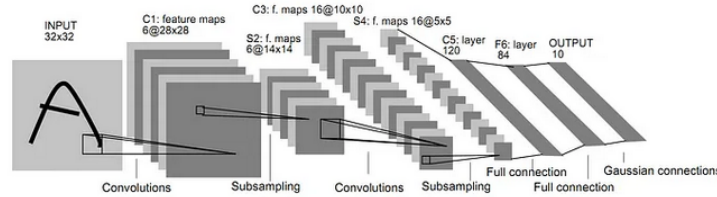
Figure 10.41: The architecture of LeNet-5, a convolutional neural network for digits recognition. Each plane is a feature map, i.e. a set of units whose weights are constrained to be identical.
