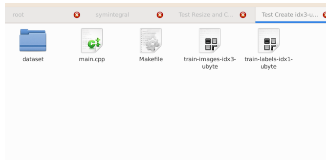
Figure 10.62: An example to create idx3-ubyte and idx1-ubyte files from two grayscale images of size 28 \times 28 (SymIntegration/Examples/Neural Networks/Test Create idx3-ubyte Files with STB Image/main.cpp).
