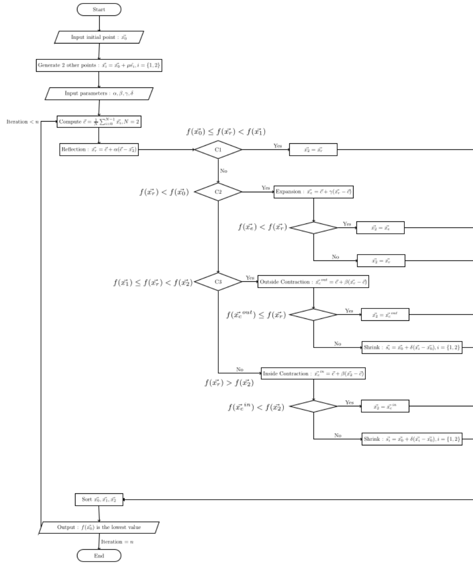
Figure 7.16: The flowchart for downhill simplex algorithm that is used to make the C++ code for computing the solution.
