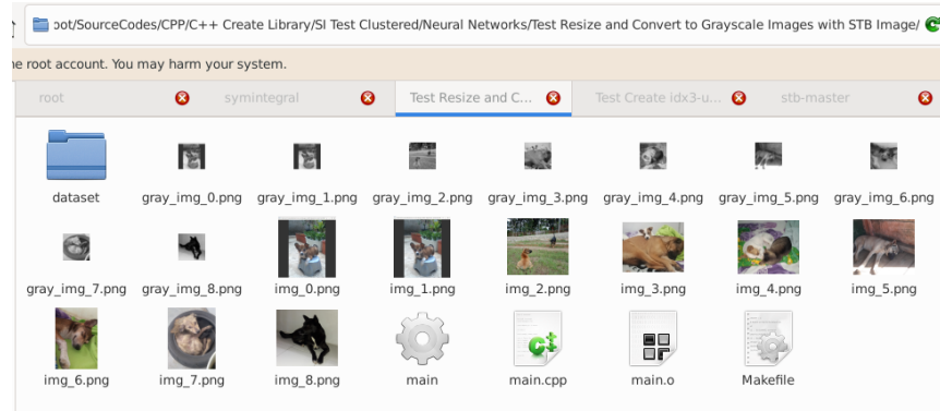
Figure 10.61: Converting several images with different sizes to uniform size of 28 \times 28 then convert them to grayscale (SymIntegration/Examples/Neural Networks/Test Resize and Convert to Grayscale Images with STB Image/main.cpp).
