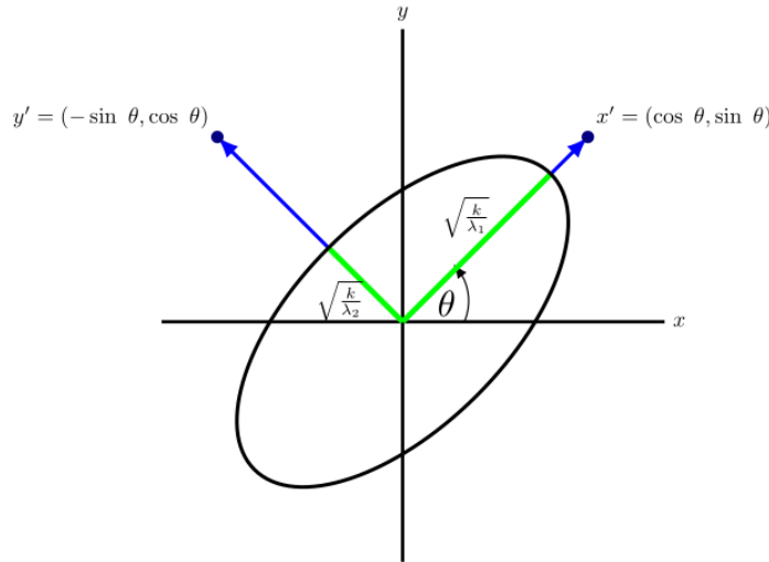
Figure 6.53: The principal axes of the ellipse, the conic above is of form \lambda_1 x'^2 + \lambda_2 y'^2 = k , if \lambda_1, \lambda_2 , and k are positive, then it is an ellipse with \alpha = \sqrt{\frac{k}{\lambda_1}} and \beta = \sqrt{\frac{k}{\lambda_2}} .
