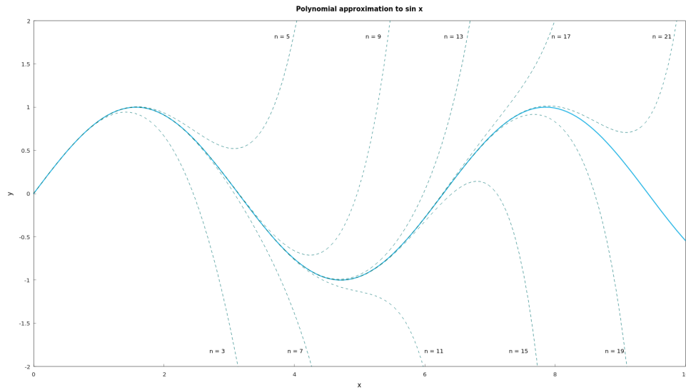
Figure 3.64: The polynomial approximations to \sin x . The value of n is the degree of the approximating polynomial (Hamzstplot/Examples with Makefile/Differential Equations/Plot 2D Polynomial Approximation to Cosine/main.cpp).
