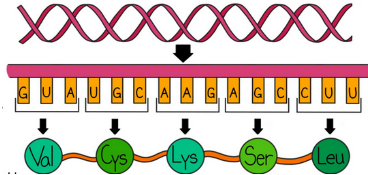
Figure 8.1: DNA is transcribed into mRNA, mRNA is translated into amino acids. Each codon corresponds to one amino acid. Amino acids form polypeptide chains. Polypeptide chains fold into proteins.
