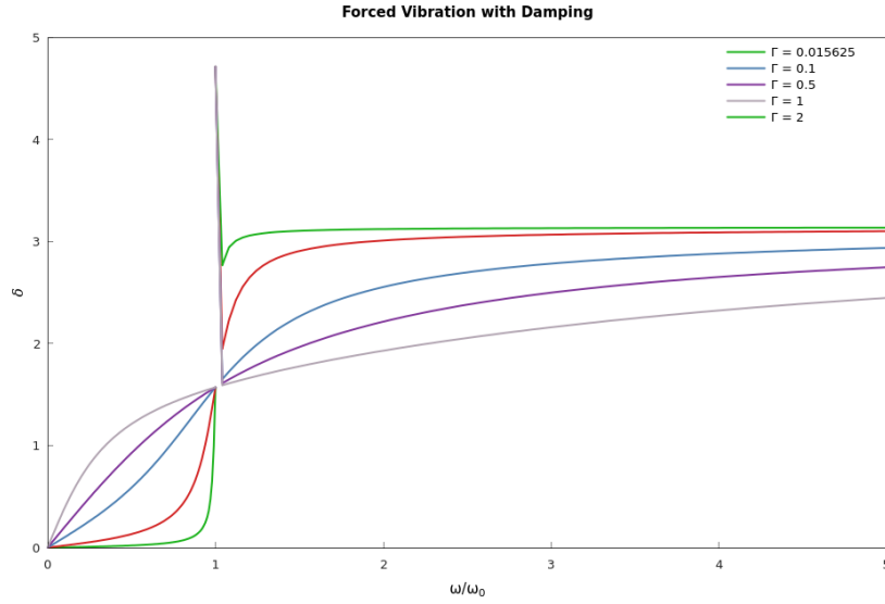
Figure 3.26: Forced vibration with damping: phase of steady state response versus frequency of driving force; \Gamma = \frac{\gamma^2}{mk} (Hamzstplot/Examples with Makefile/Differential Equations/Plot 2D Forced Vibrations Phase of Steady State Response versus Frequency of Driving Force/main.cpp).
