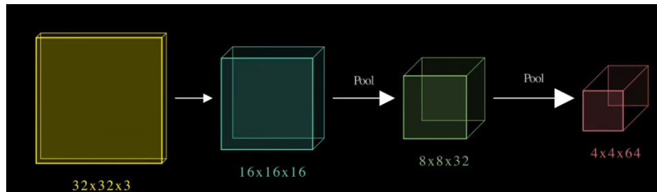
Figure 10.28: The spatial dimensions gradually get smaller while the depth / the number of channels grows. The early layers work with large spatial maps and few channels, while the deeper layers work with small spatial maps and many channels.
