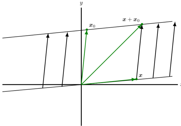
Figure 6.59: T(\mathbf{x}) = \mathbf{x} + \mathbf{x}_0 translates each point \mathbf{x} along a line parallel to \mathbf{x}_0 through a distance \|\mathbf{x}_0\| .
