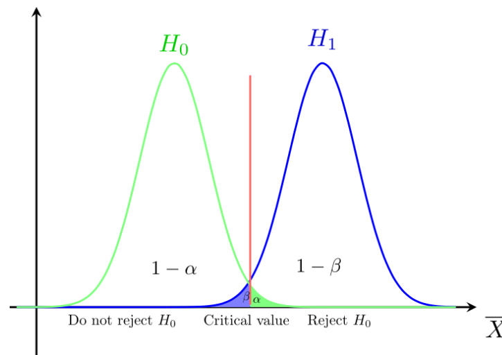
Figure 4.28: Probability of type I and type II errors.
