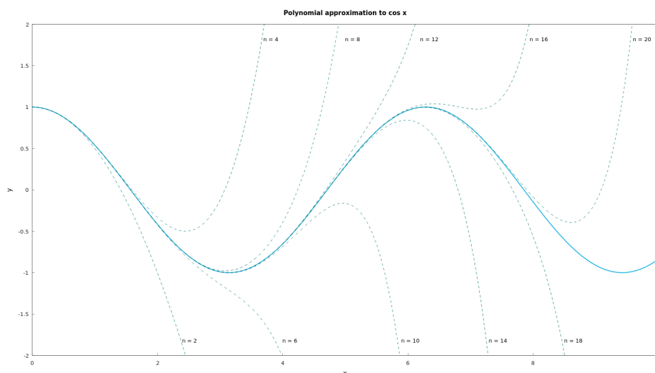
Figure 3.63: The polynomial approximations to \cos x . The value of n is the degree of the approximating polynomial (Hamzstplot/Examples with Makefile/Differential Equations/Plot 2D Polynomial Approximation to Cosine/main.cpp).
