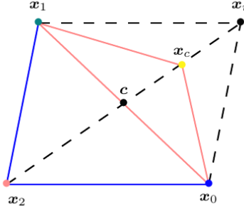
Figure 7.13: The contraction point x_c^{out} is computed outside the old simplex.
