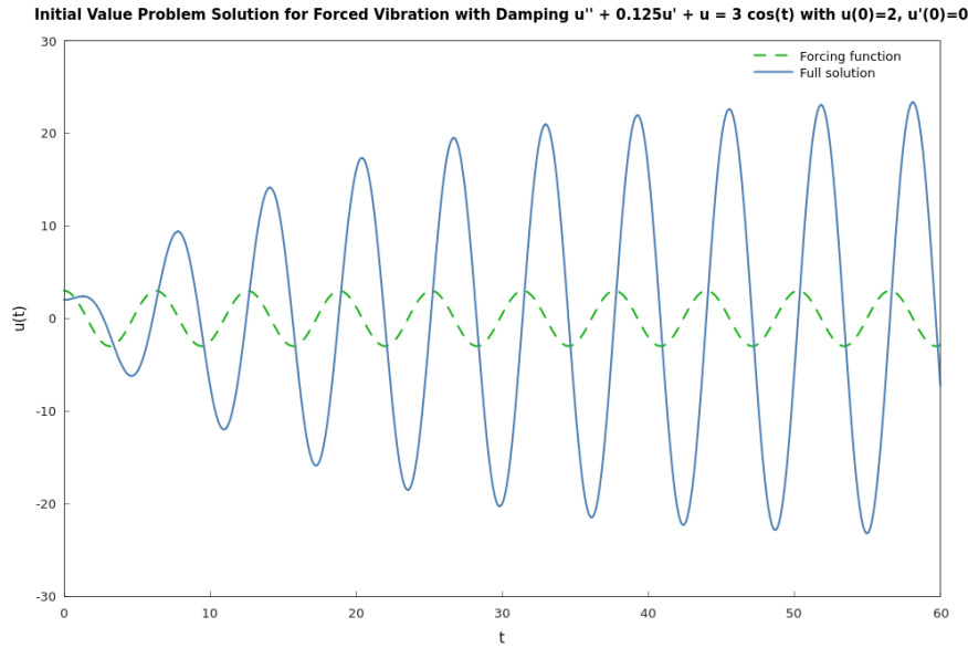
Figure 3.37: A forced vibration with damping; solution of u'' + 0.125u' + u = 3 \cos t, u(0) = 2, u'(0) = 0 (Hamzstplot/Examples with Makefile/Differential Equations/Plot 2D Forced Vibrations IVP Second Order ODE Solution and Forcing Function/main.cpp).
