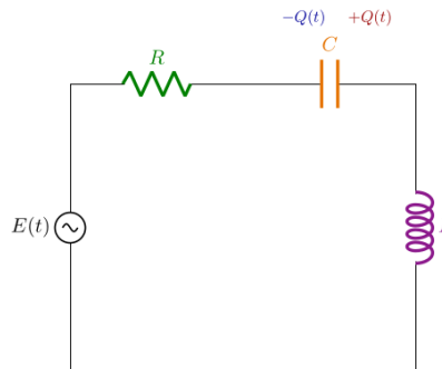
Figure 3.22: A simple RLC series electric circuit.
