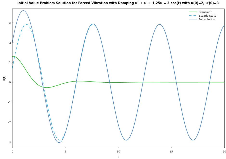
Figure 3.24: The graph of the solution (3.187) for the initial value problem for the second order nonhomogeneous differential equation ( Hamzstplot/Examples with Makefile/Differential Equations/Plot 2D Forced Vibrations IVP Second Order ODE/main.cpp ).
