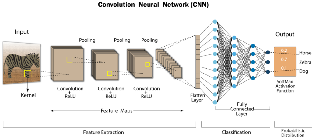
Figure 10.23: The illustration of convolutional neural network pipeline for image classification.
