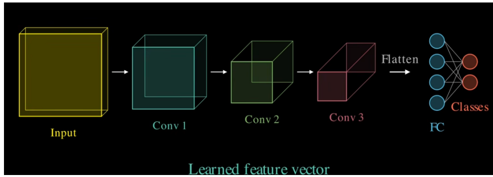
Figure 10.27: After the last convolution layer, we will flatten the 3D matrix into a vector then process it again till the output layer that produces the probability for the image classification.
