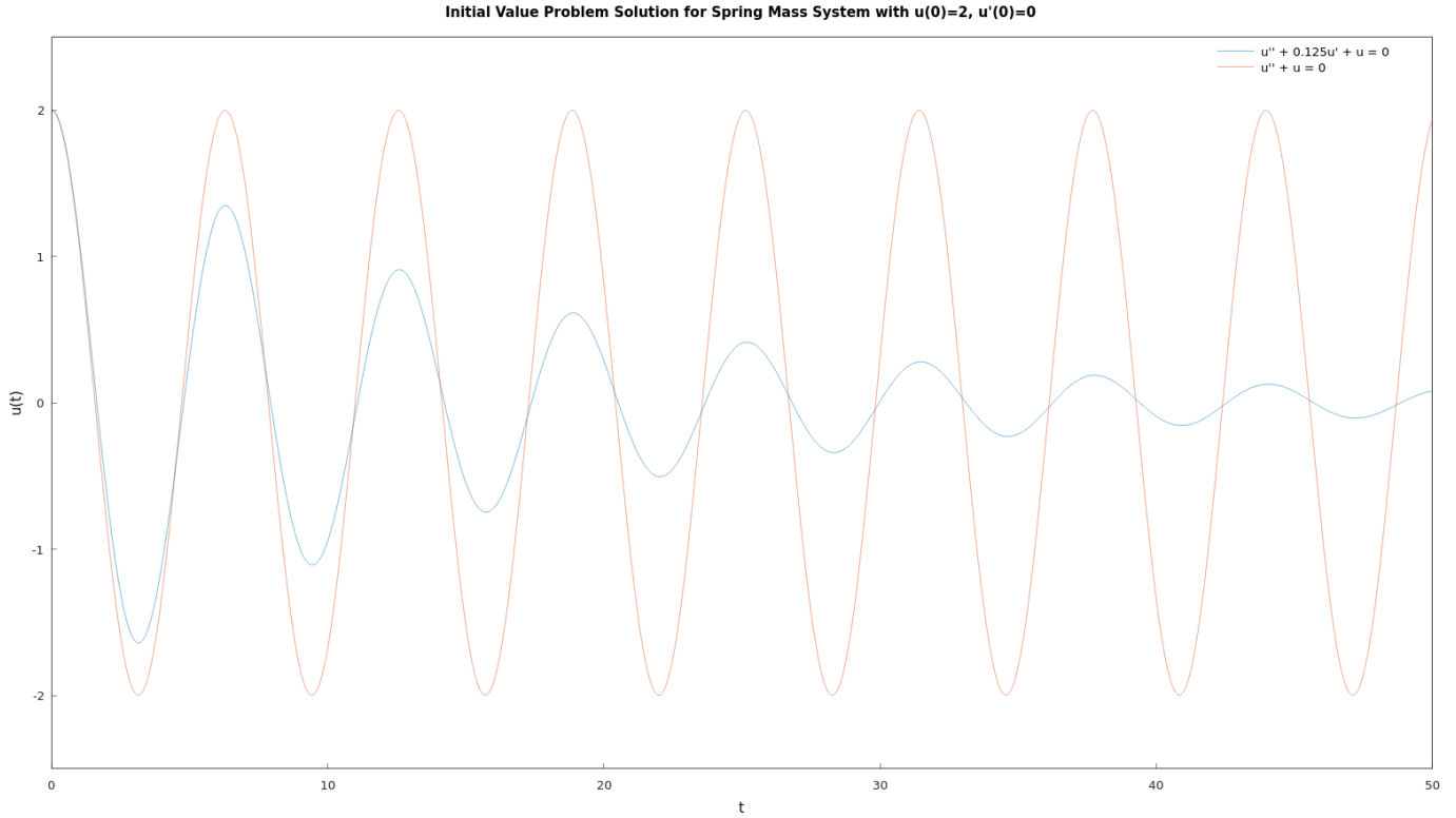
Figure 3.20: The figure shows the displacement of the mass as a function of time. For purposes of comparison, we also show the motion if the damping term is neglected. ( Hamzstplot/Examples with Makefile/Differential Equations/Plot 2D Vibration with Small Damping and With No Damping Second Order ODE/main.cpp ).
