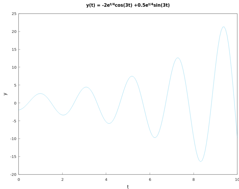
Figure 3.14: The graph of the solution y = -2e^{t/4} \cos 3t + \frac{1}{2}e^{t/4} \sin 3t of the initial value problem 16y'' - 8y' + 145y = 0, y(0) = -2, y'(0) = 1 (Hamzstplot/Examples with Makefile/Differential Equations/Plot 2D Growing Oscillation/main.cpp).
