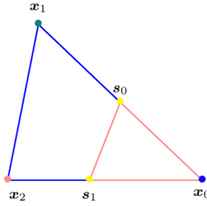
Figure 7.15: Shrink the simplex by moving every point closer to the current best.
