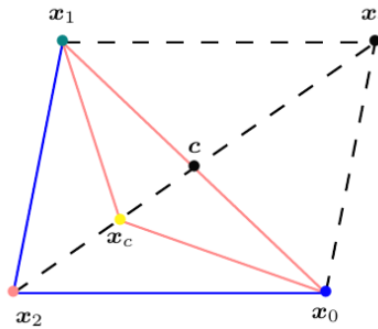
Figure 7.14: The contraction point x_c^{in} is computed inside the old simplex.
