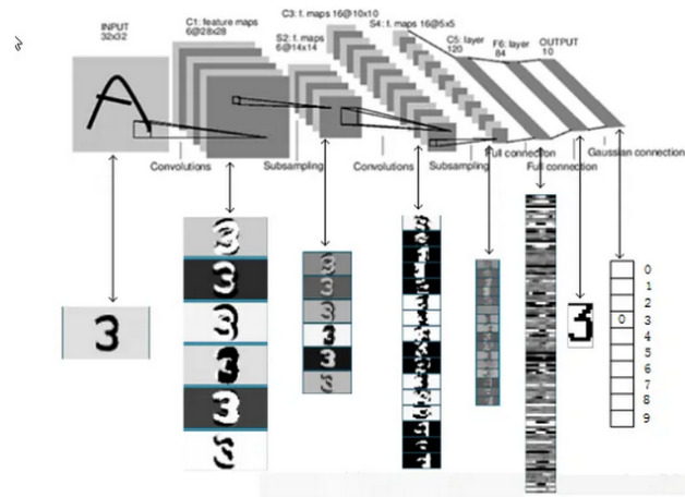
Figure 10.44: The LeNet-5 architecture & pipeline for digit recognition. It is a very efficient convolutional neural network for handwritten character recognition.
