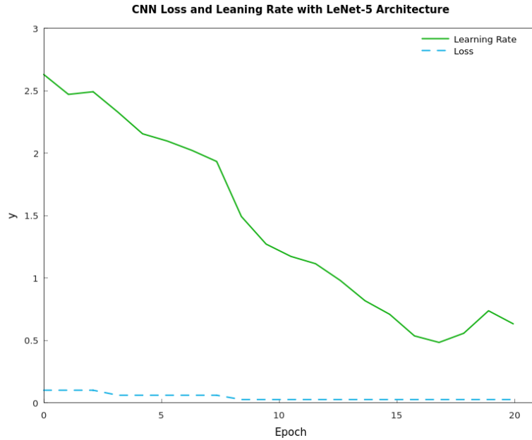
Figure 10.49: The training loss of LeNet-5 as plotted over 20 epochs along with the learning rate at each epoch. The training loss is monotonically decreasing indicating the network is effectively learning to differentiate between the ten classes in the dataset ( Hamzstplot/Examples with Makefile/Neural Networks/Plot 2D Line for Loss and Learning rate for CNN/main.cpp ).
