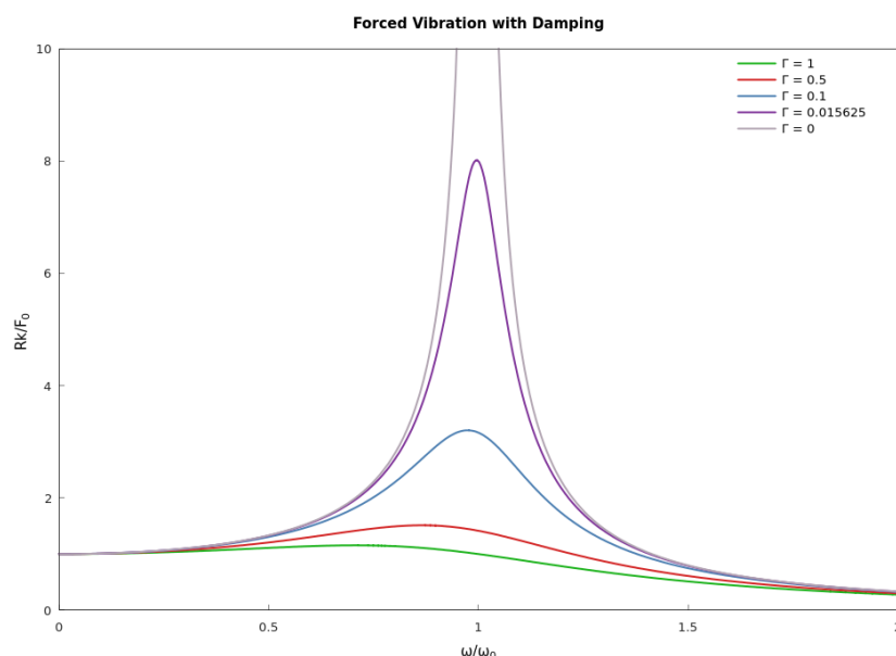
Figure 3.25: Some representative graphs of \frac{Rk}{F_0} versus \frac{\omega}{\omega_0} for several values of \Gamma = \frac{\gamma^2}{mk} (Hamzstplot/Examples with Makefile/Differential Equations/Plot 2D Forced Vibrations Amplitude of Steady State Response versus Frequency of Driving Force/main.cpp).
