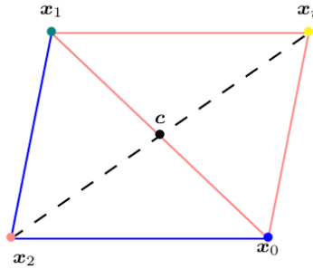
Figure 7.11: x_2 is mirrored in c and creates a reflected point x_r .
