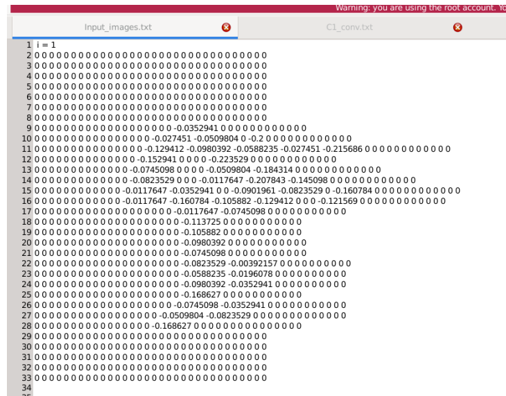
Figure 10.48: The normalized input image with range [-1, 1] and we also notice that the background paper has positive value while the pen stroke has negative value, thus we zeroes all the positive values and let the negative values be.
