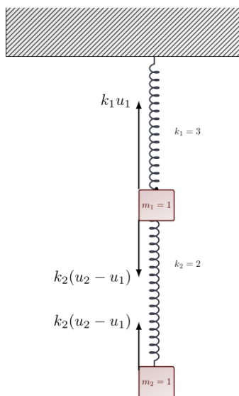
Figure 3.46: A two-spring, two-mass system.
