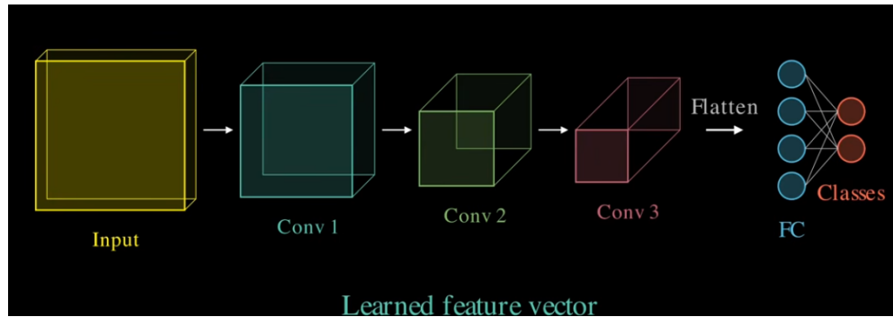
Figure 10.27: After the last convolution layer, we will flatten the 3D matrix into a vector then process it again till the output layer that produces the probability for the image classification.
