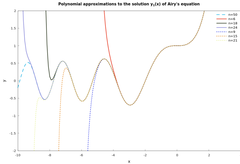
Figure 3.65: The polynomial approximations to the solution y_1(x) of Airy's equation. The value of n is the degree of the approximating polynomial (Hamzstplot/Examples with Makefile/Differential Equations/Plot 2D Solution of Airy's Equation Ai(x)/main.cpp).
