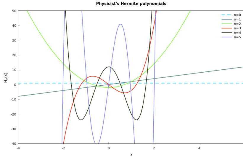
Figure 3.80: The physicist's Hermite polynomials ( Hamzstplot/Examples with Makefile/Differential Equations/-Plot 2D Physicist's Hermite Polynomials/main.cpp ).
