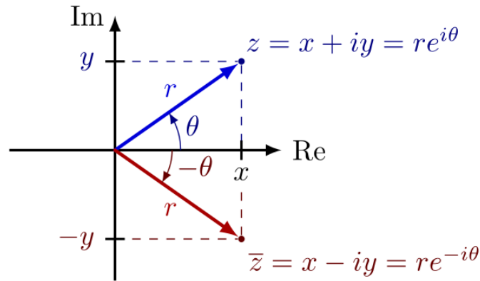
Figure 2.7: The complex number can be represented as z = x + iy = re^{i\theta} , with r = |z| and the angle \theta is the argument of z .
