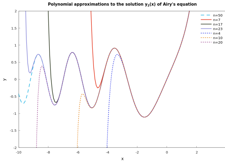
Figure 3.66: The polynomial approximations to the solution y_2(x) of Airy's equation. The value of n is the degree of the approximating polynomial (Hamzstplot/Examples with Makefile/Differential Equations/Plot 2D Solution of Airy's Equation Bi(x)/main.cpp).
