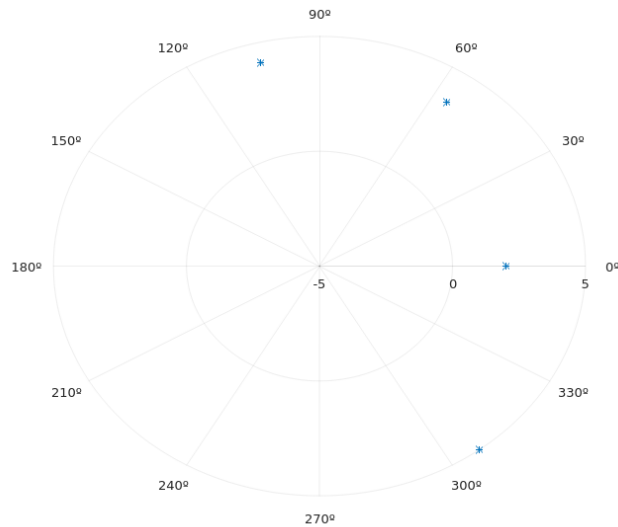
Figure 2.8: The polar plot of several complex numbers: 2 + 3i, -1 + 4i, 3 - 4i (Hamzstplot/Examples with Makefile/Complex Analysis/Plot 2D Complex Numbers/main.cpp).
