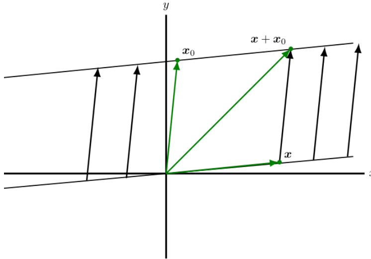
Figure 6.59: T(x) = x + x_0 translates each point x along a line parallel to x_0 through a distance \|x_0\| .
