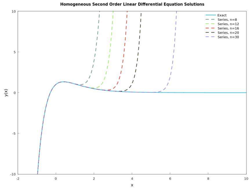
Figure 3.73: The plot of the exact solution and the series solution with various terms for the differential equation y'' + 3y' + 2y = 0 , we combine SymIntegration library with Hamzstplot, thus SymIntegration is used to compute the series solution and then plot it with Hamzstplot ( Hamzstplot/Examples with Makefile/Differential Equations/Plot 2D Comparing Series Solutions with Exact Solution for Second Order Homogeneous Linear Differential Equation/main.cpp ).
