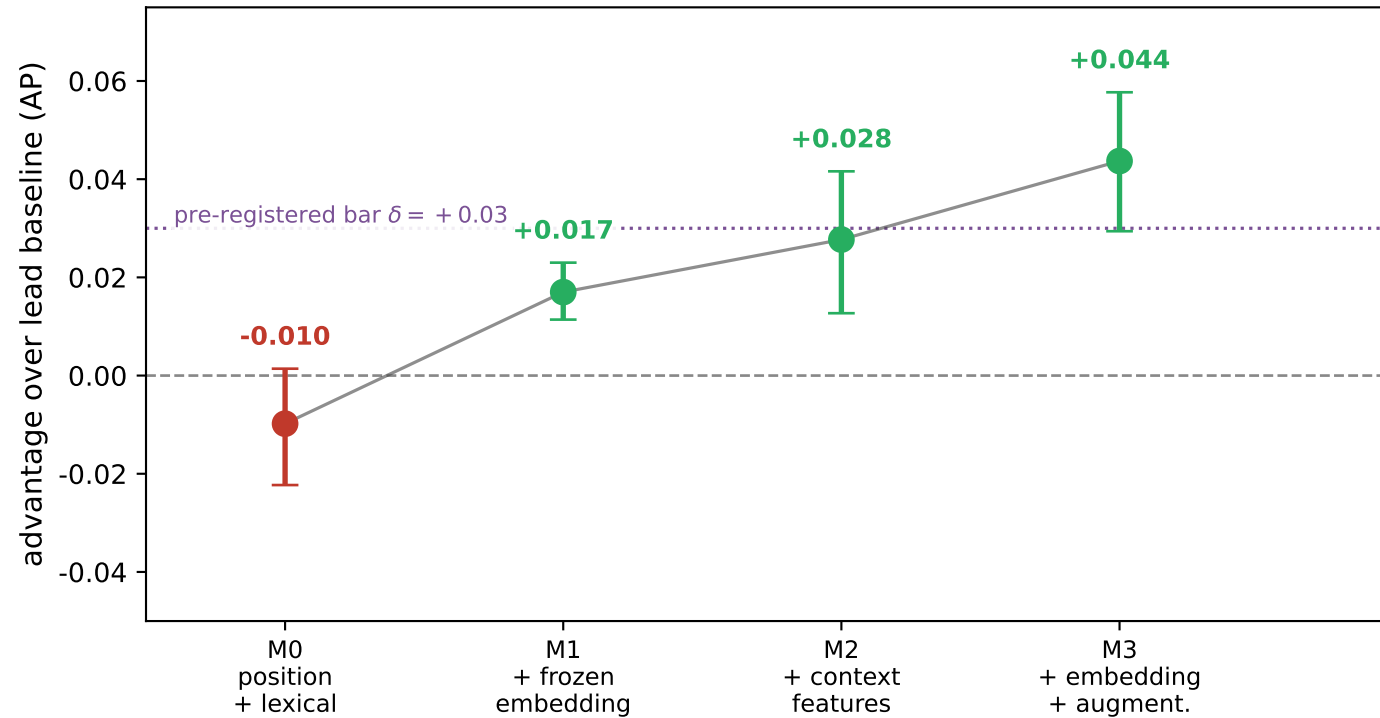
A trained model's edge over position grows with representation (crosses the pre-registered bar at M3)
