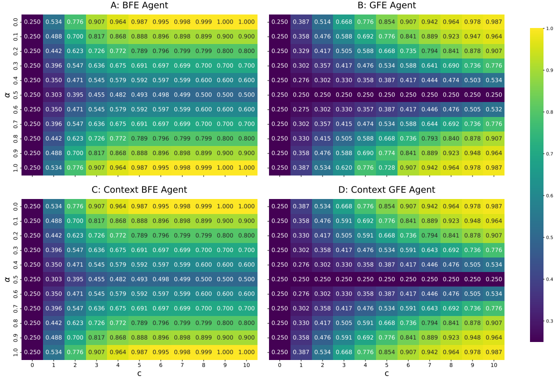
Figure 3.2: Inferred probabilities of moving to the arm in the T-Maze that is hinted by the cue to contain the reward for the four agents (BFE, GFE, Context-BFE, and Context-GFE) with differing \alpha - and c values.
