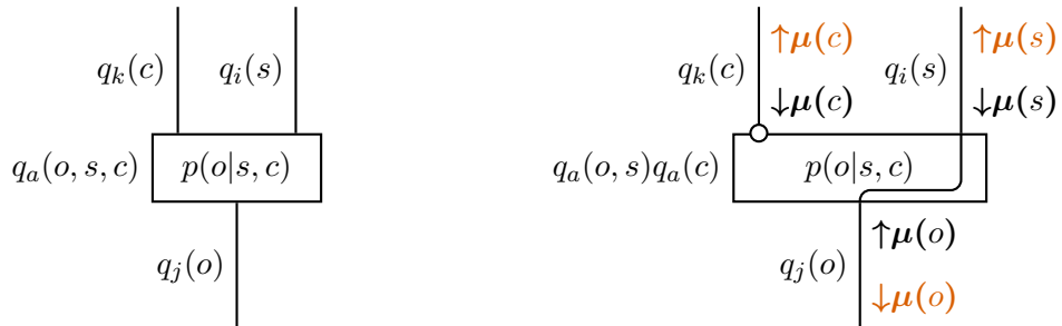
(a) Factor node with node belief that respects variables' dependencies.
