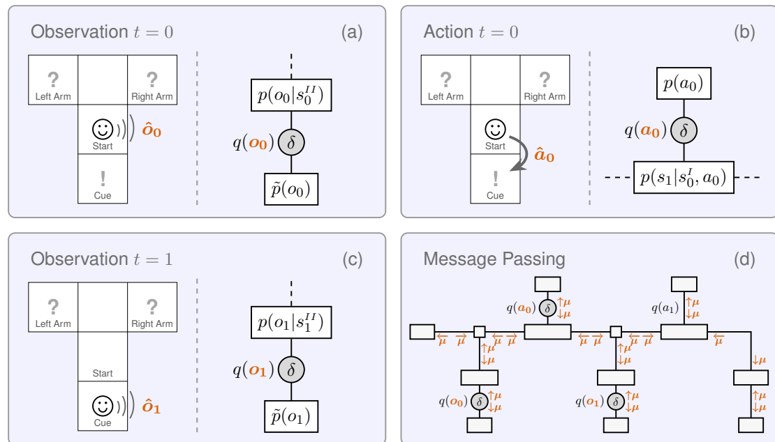
Figure 2.22.: The figure presents the four steps of Experiment 2 via the example of the BFE agent. First, the agents receives an observation \hat{o}_0 which makes q(o_0) a delta distribution with all its probability mass at \hat{o}_0 (a). Second, the action "go to cue" is externally triggered and the respective belief distribution q(a_0) also becomes a delta distribution with its mass at this action (b). Third, being at the cue triggers an observation from the environment that is informative regarding the reward location. Similar to the first observation, it leads to a delta distribution at q(o_1) (c). Lastly, the agent executes its message passing algorithm to infer all its belief distributions (d). The inclination of moving to the cued arm that promises the reward is then given as a probability in the action-specific belief distribution q(a_1) .
