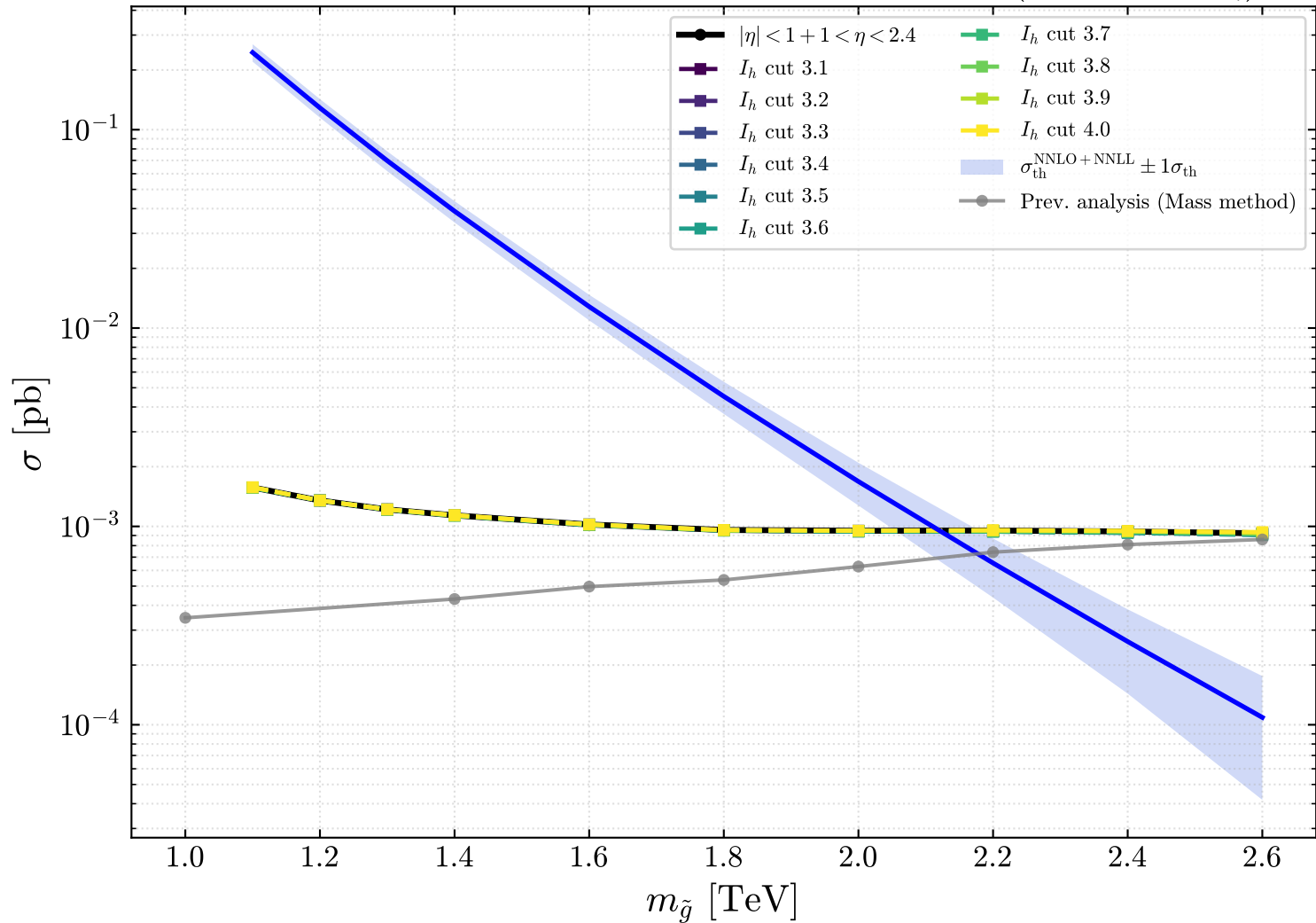
Expected median limits – gluino R-hadron, 2024 (shape, split \eta )
