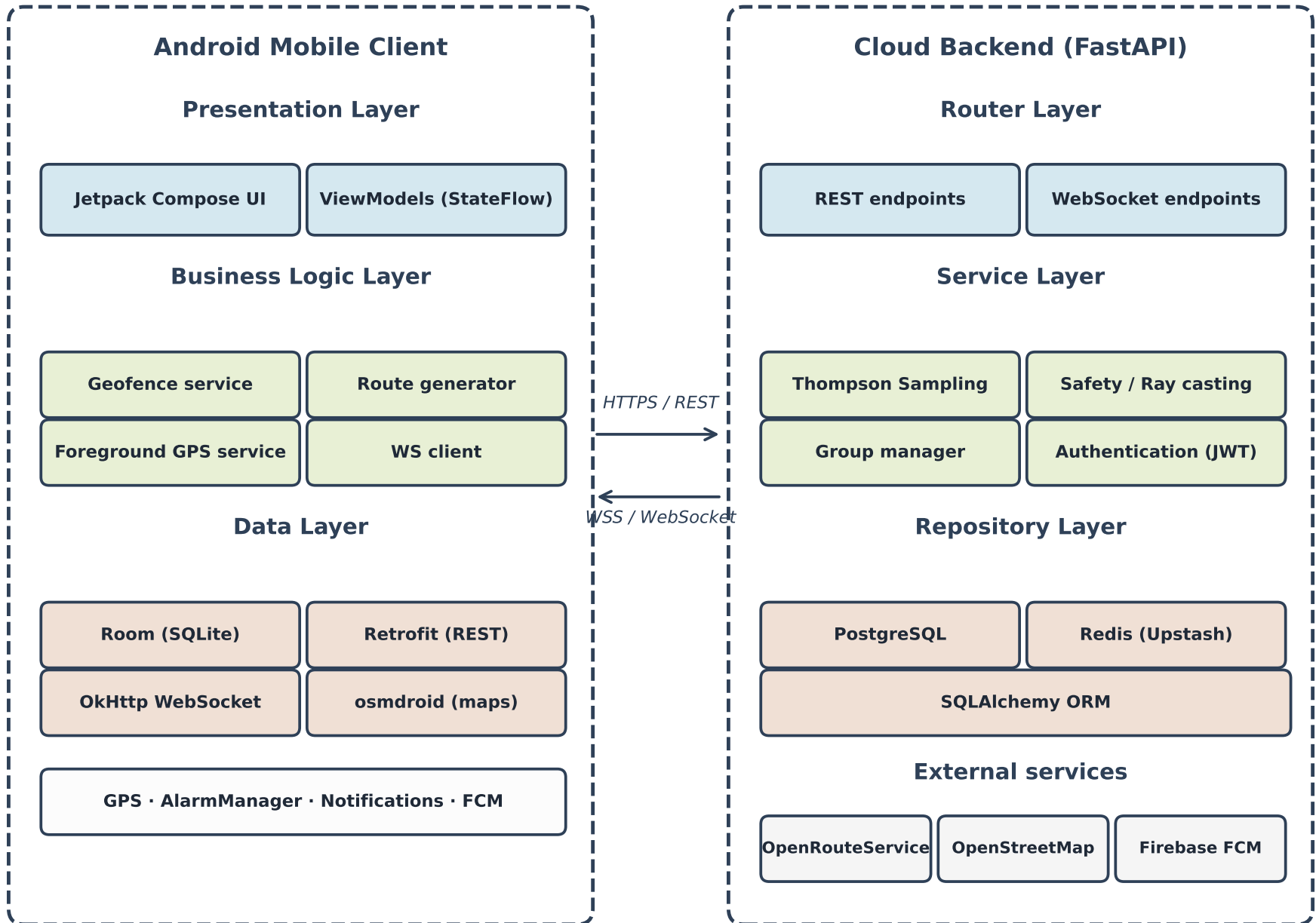
Figure 1. System architecture of RutAI — three-layer client-server design
