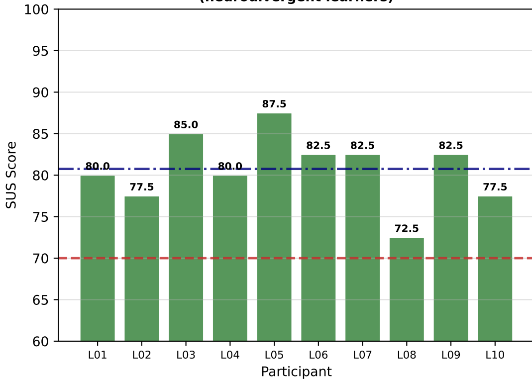
Individual SUS Scores (neurodivergent learners)
