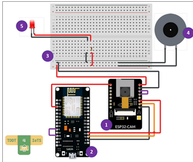
Fig. 6: Design of the IoT device of the Torddis system.
