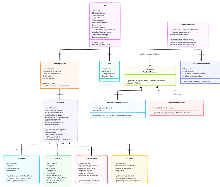
Figura 2.3: UML class diagram of the main components. Source: Own elaboration.
