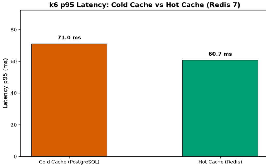
Figure 8.1: Comparative latency distribution of the k6 runs. Source: Own elaboration.
