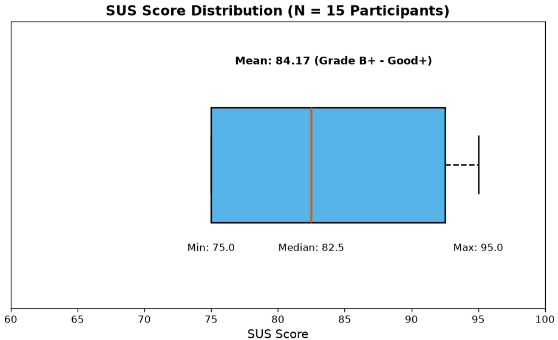
Figura 8.2: SUS score distribution and individual scores for 15 participants. Source: Own elaboration.
