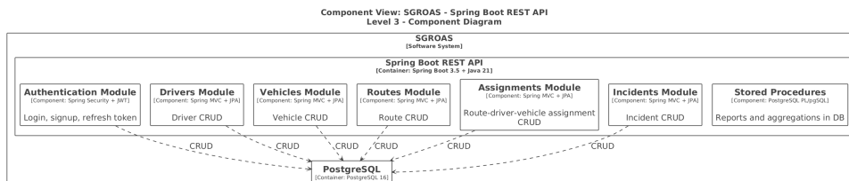
Figure 6.3: C4 Level 3 Diagram — SGROAS Backend Components.
