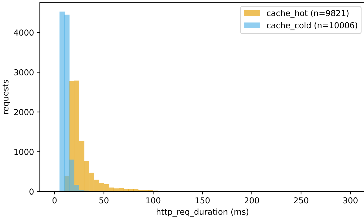
Latency distribution: cache_hot vs cache_cold (5 runs)
