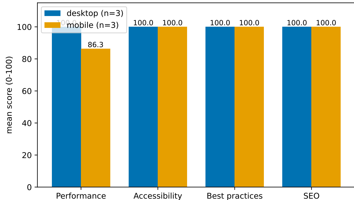
Lighthouse post-fix means: desktop vs mobile (prod, 2026-08-18)
