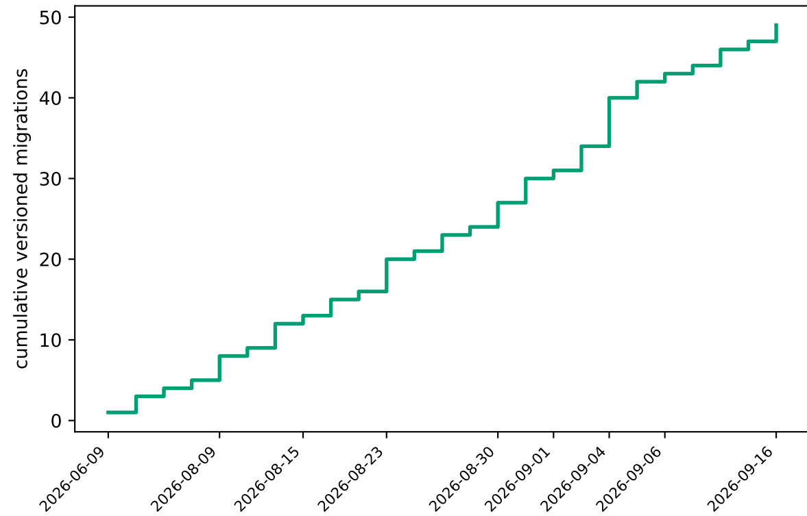
Flyway migrations over time (49 versioned V-files)
