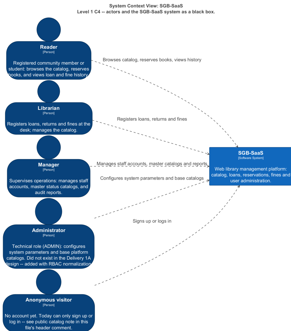
Figura 6.1: C4 model, Level 1 (System Context): the five system actors and their interactions with SGB-SaaS as a black box. Exported automatically from workspace.dsl .
