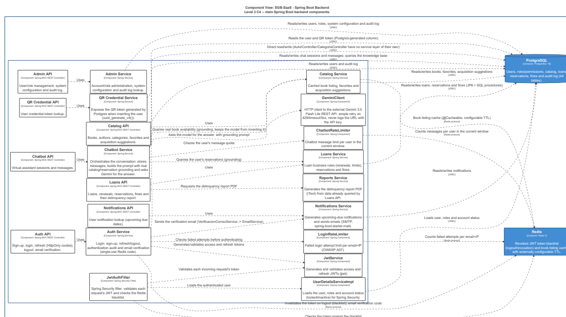
Figura 6.4: C4 model, Level 3 (Components) for the Spring Boot backend – 21 components grouped by domain (API layer, service layer, security, and external integration), with relationships verified against the real codebase. PDF conversion from the versioned source SVG at docs/arquitectura/c4-nivel3-componentes.svg .
