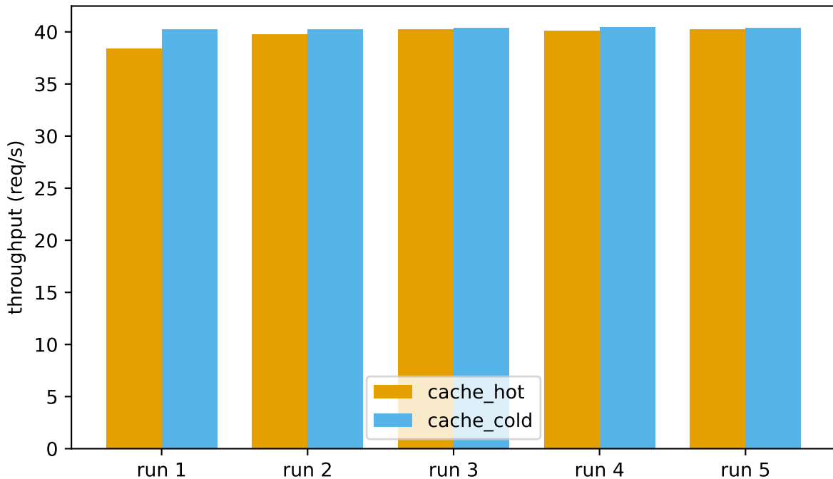
Throughput per run and scenario (GET /api/v1/libros)
