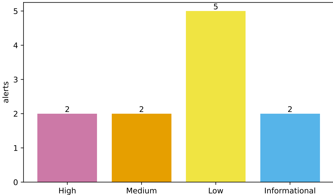
ZAP AJAX spider alerts by risk (2026-08-17, 11 alerts)
