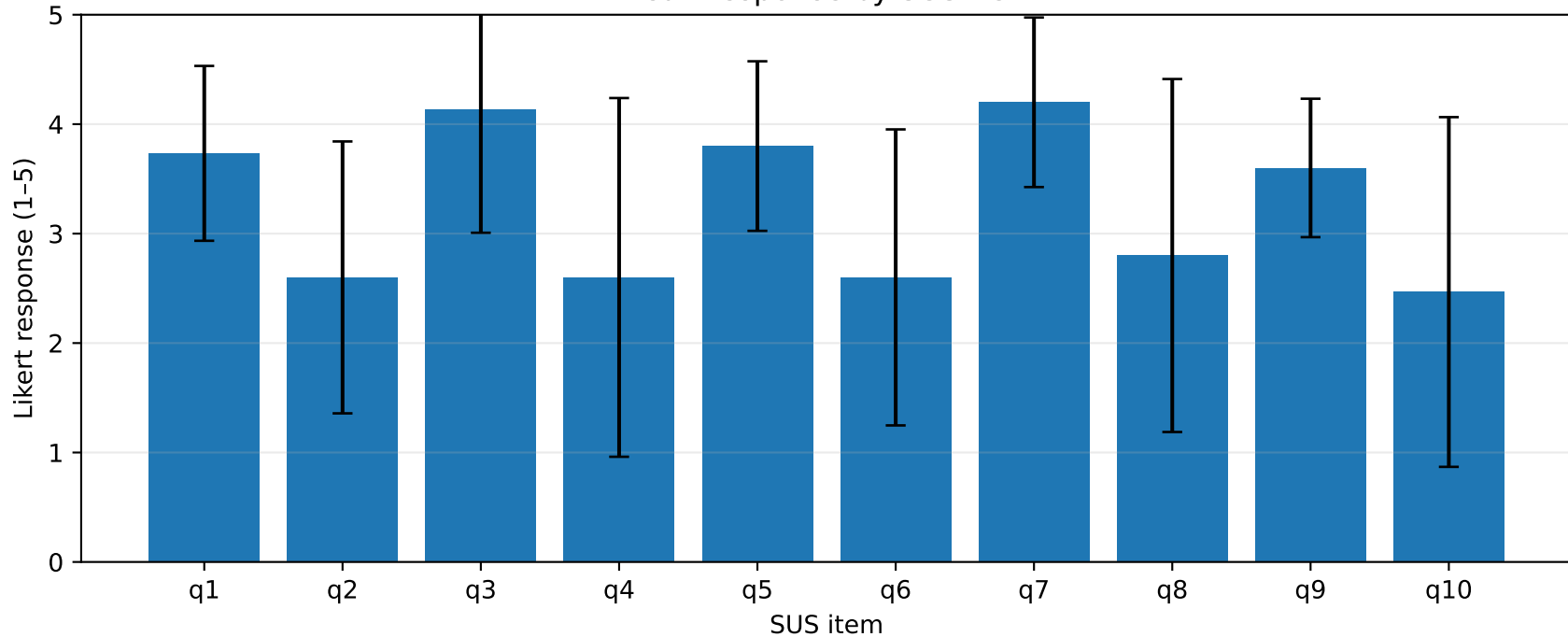
Mean response by SUS item
