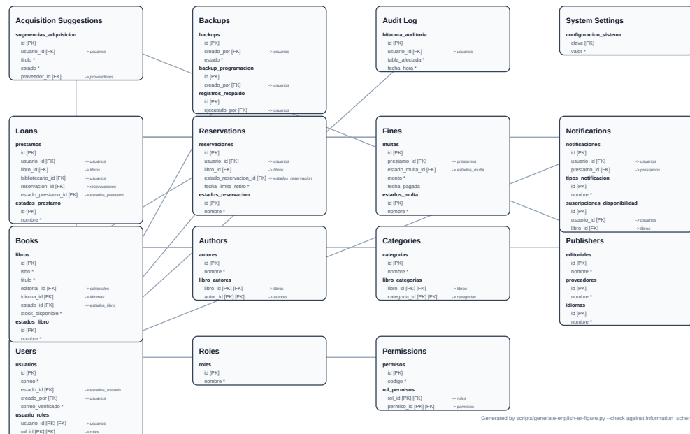
Figura 6.3: Entity relationship overview with English area labels: real tables and key columns with PK/FK marks and cardinalities, generated from a spec verified against the PostgreSQL schema. Full table-level detail with real identifiers in docs/diagramas/der-real.pdf.
