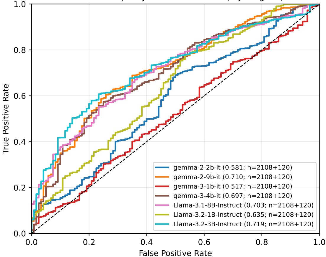
AAG - Prompt Injection Detection (InjecAgent)
