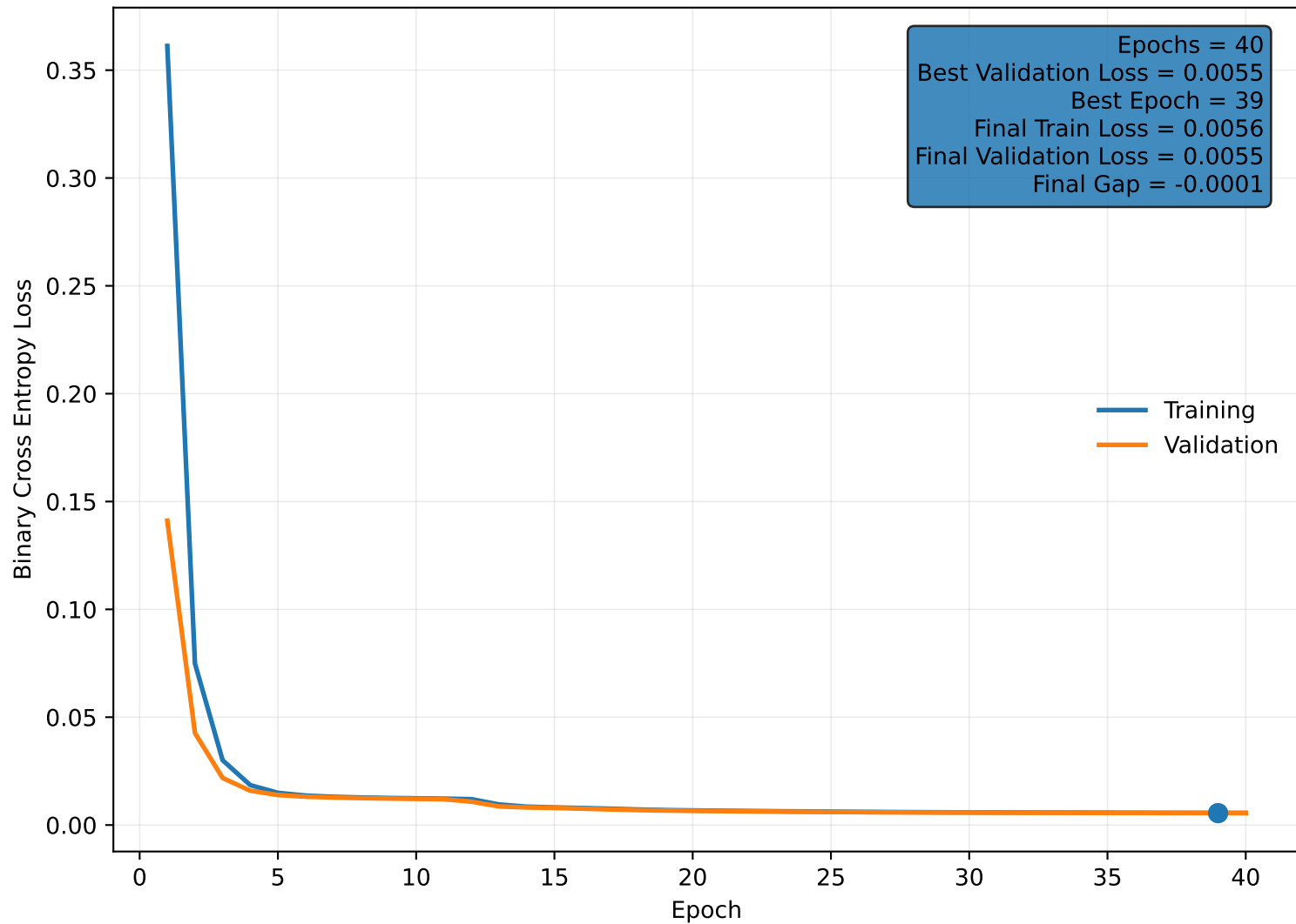
Segmentation Training History
