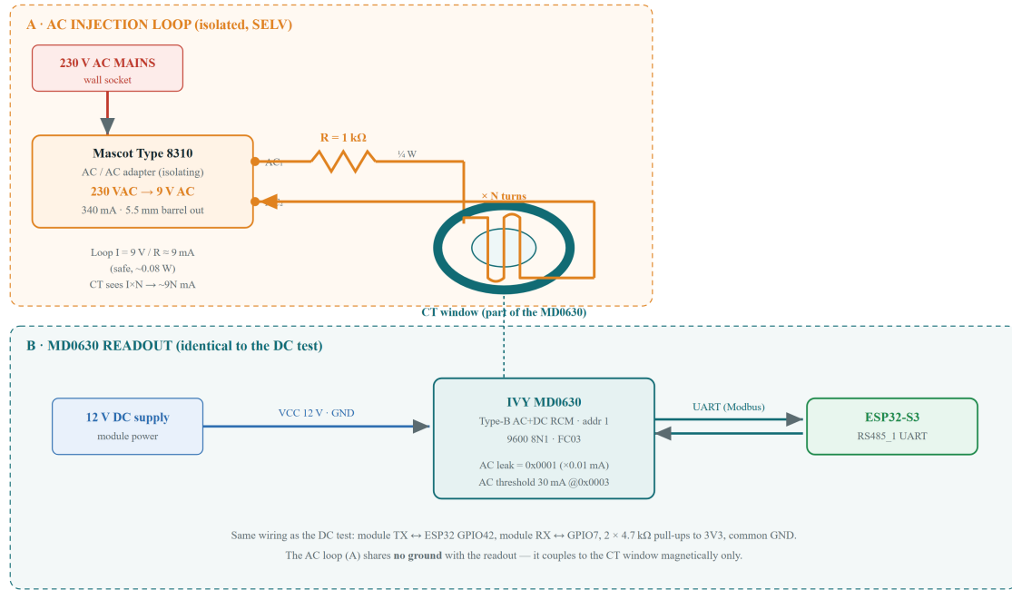
Figure 9: AC leakage test wiring: an isolated 9 V AC source drives a 1 k \Omega resistor and a wire threaded N turns through the CT window; the readout is identical to the DC test.
