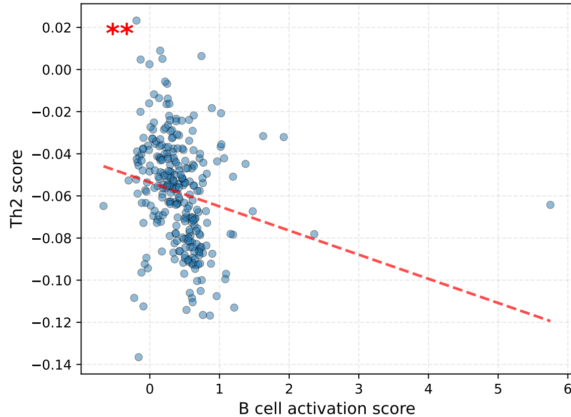
Th2 vs B cell activation Spearman r=-0.368 , p=2.089\text{e-}10 , n=280
