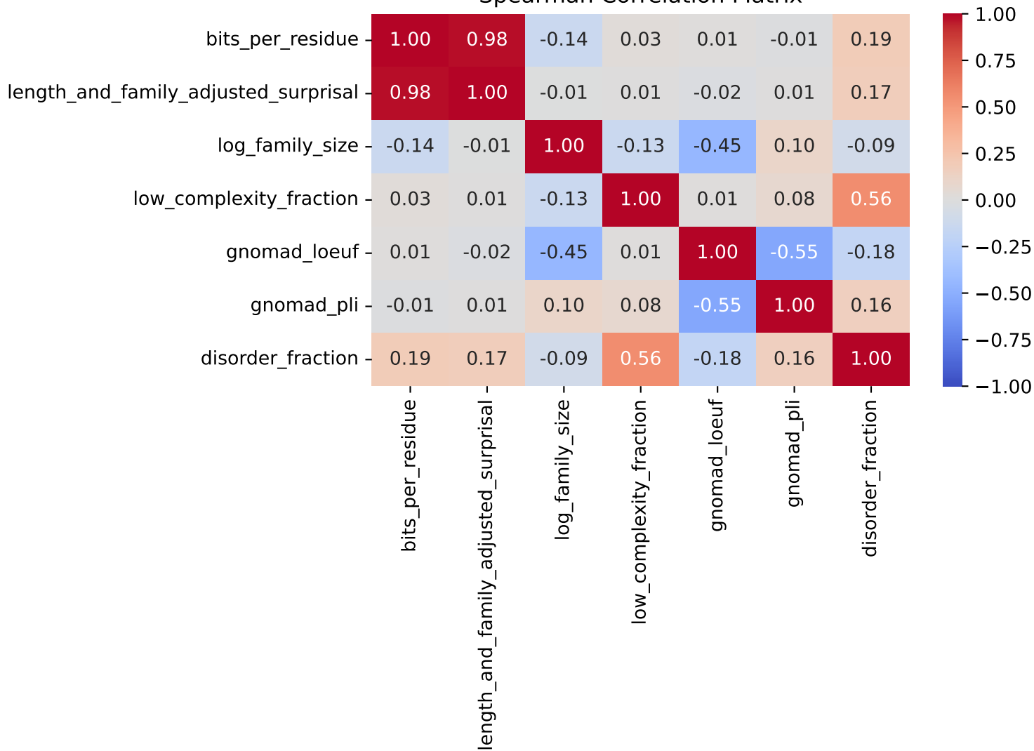
Spearman Correlation Matrix
