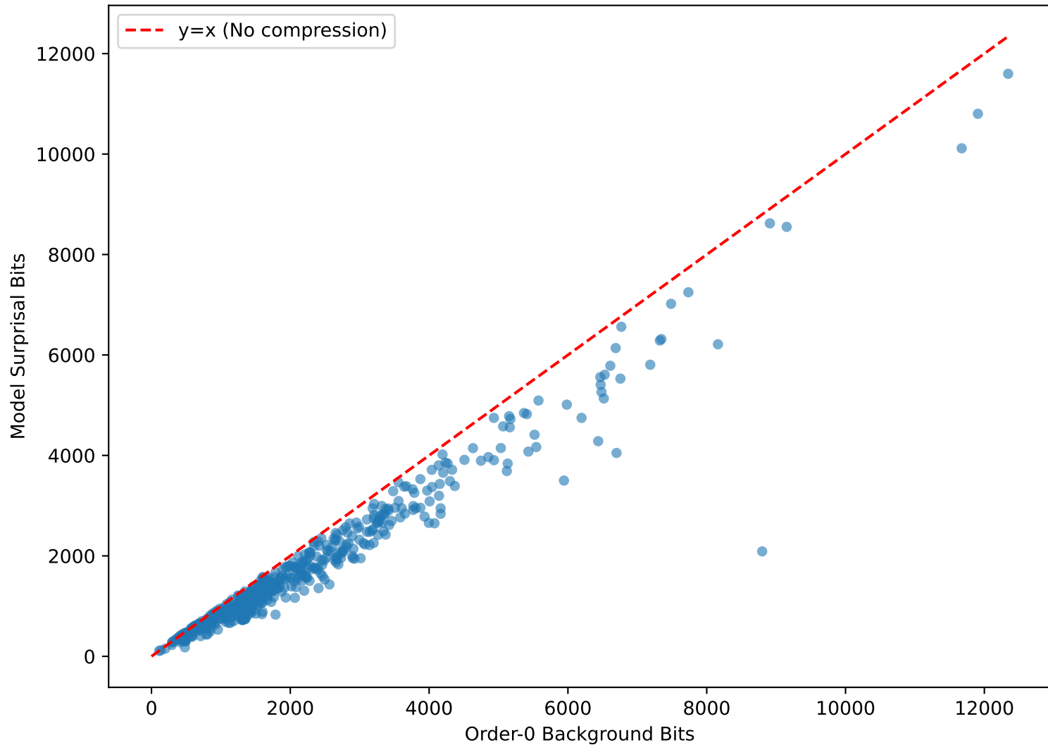
Background Bits vs Model Surprisal
