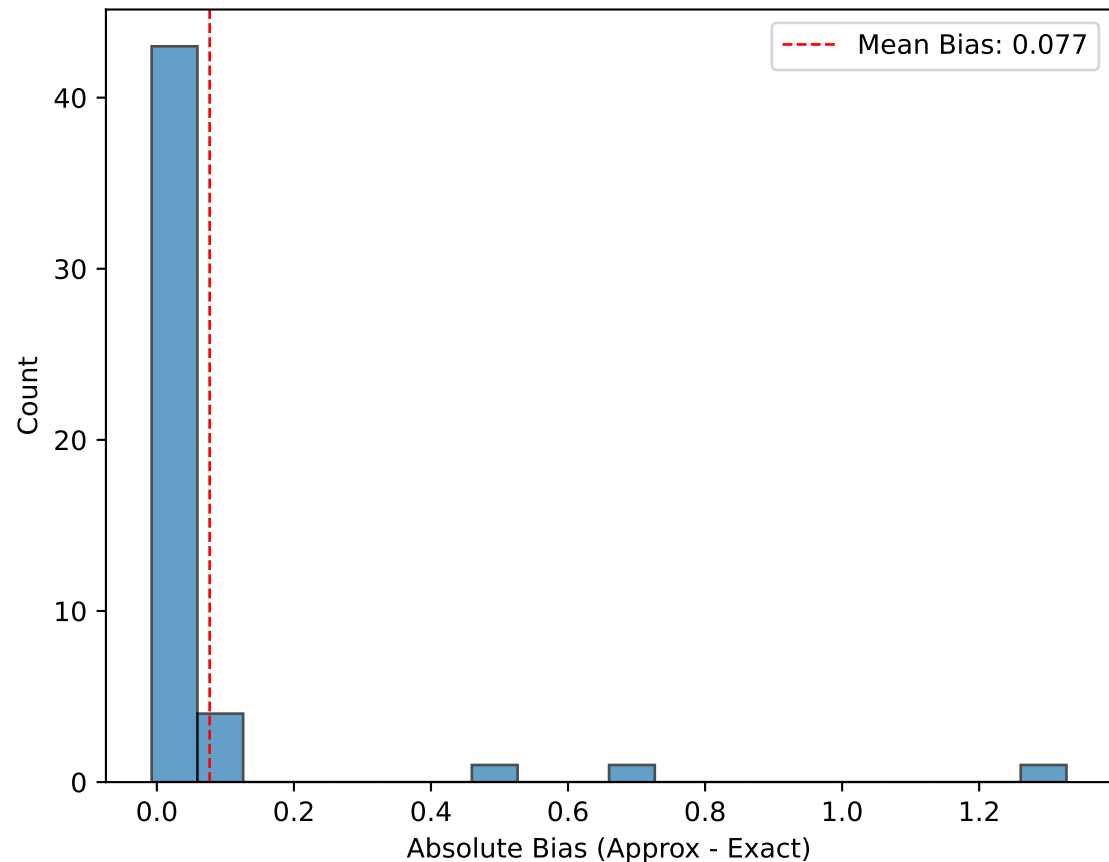
Absolute Bias Distribution
