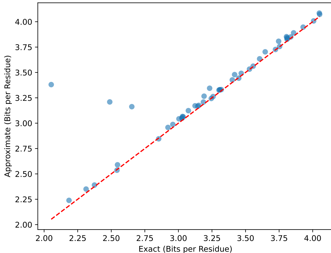
Scoring Validation (Spearman \rho=0.94 )
