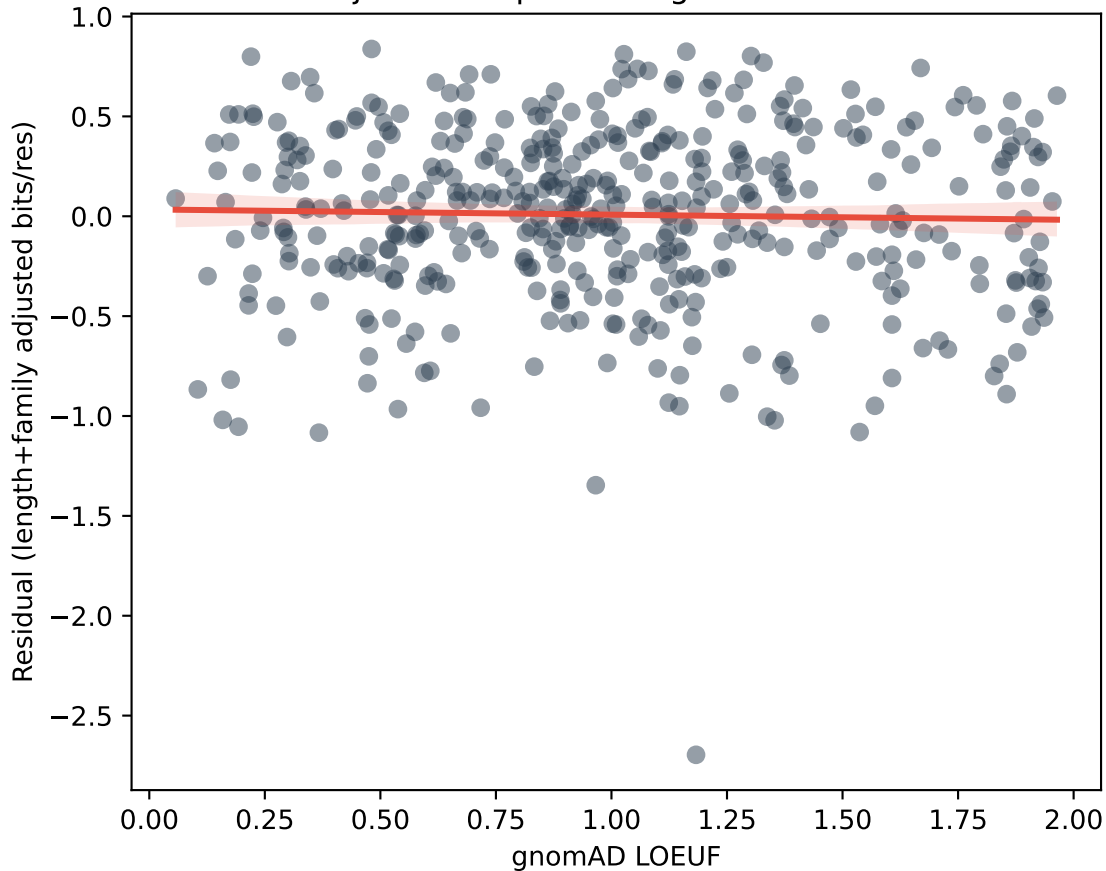
Adjusted Surprisal vs. gnomAD LOEUF
