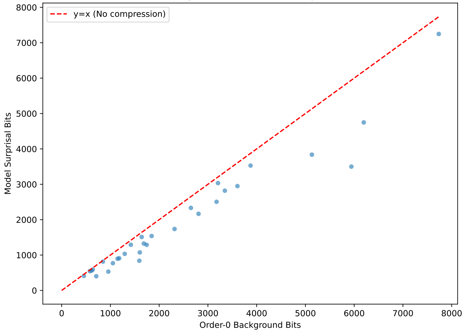
Background Bits vs Model Surprisal
