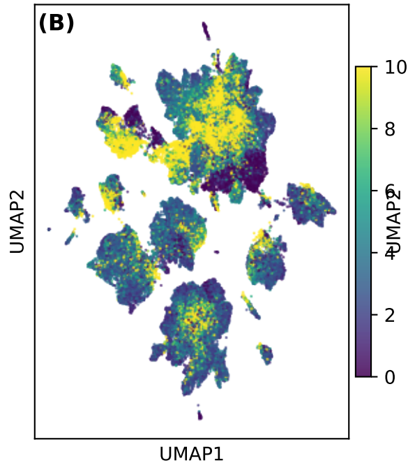
Mitochondrial RNA (%)
