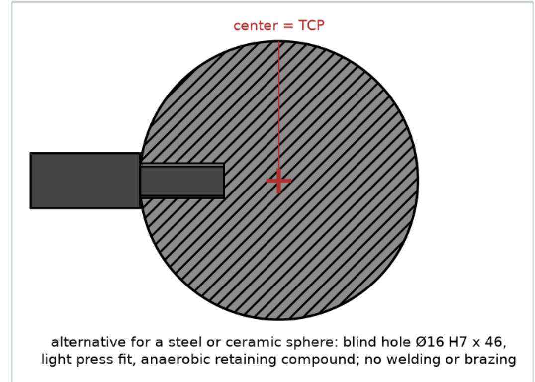
Steel or ceramic alternative: bonded blind hole
