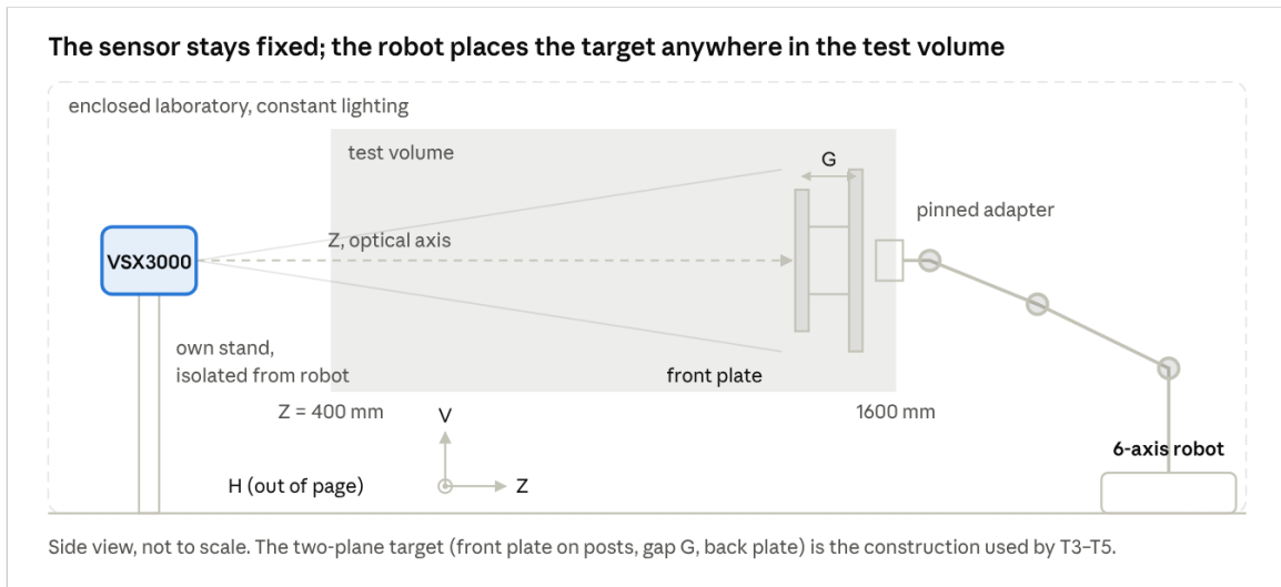
Figure 3. Experimental setup, side view
