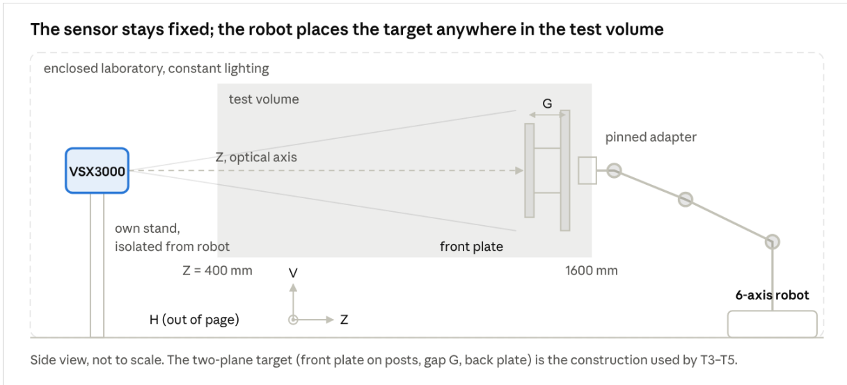
Figure 3. Experimental setup, side view
