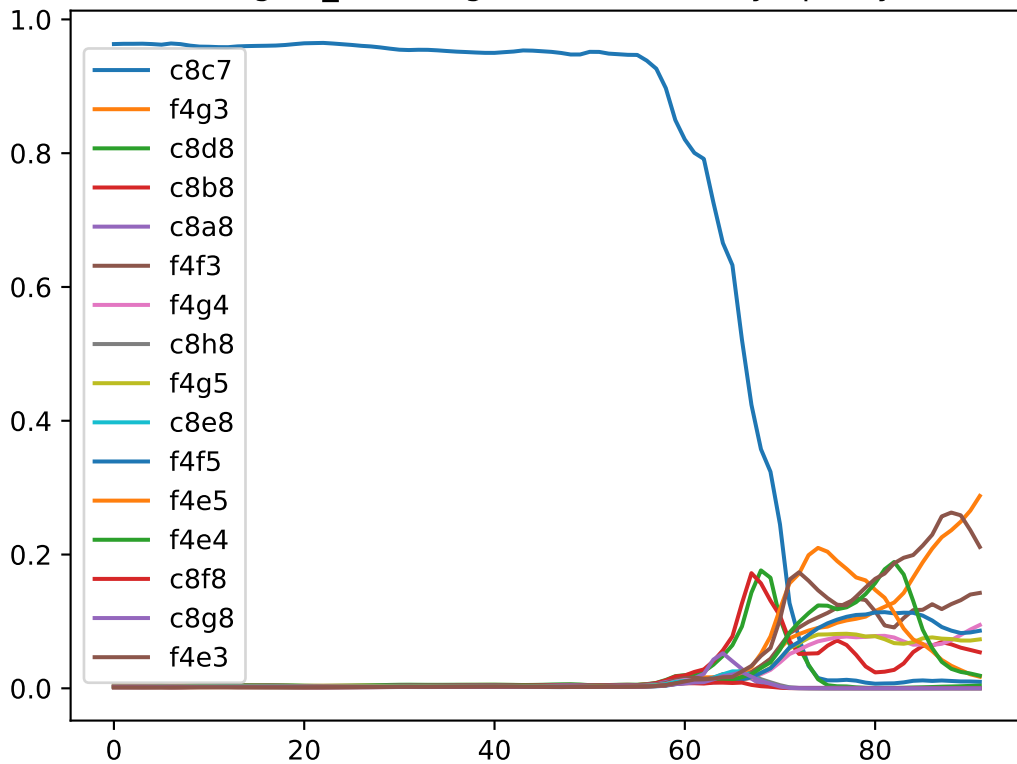
weights_288.txt.gz - Normal history - policy
