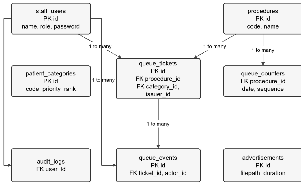
Figure 8. Relationships declared in the SQL schema
