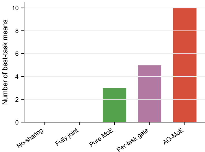
Best mean performance count
