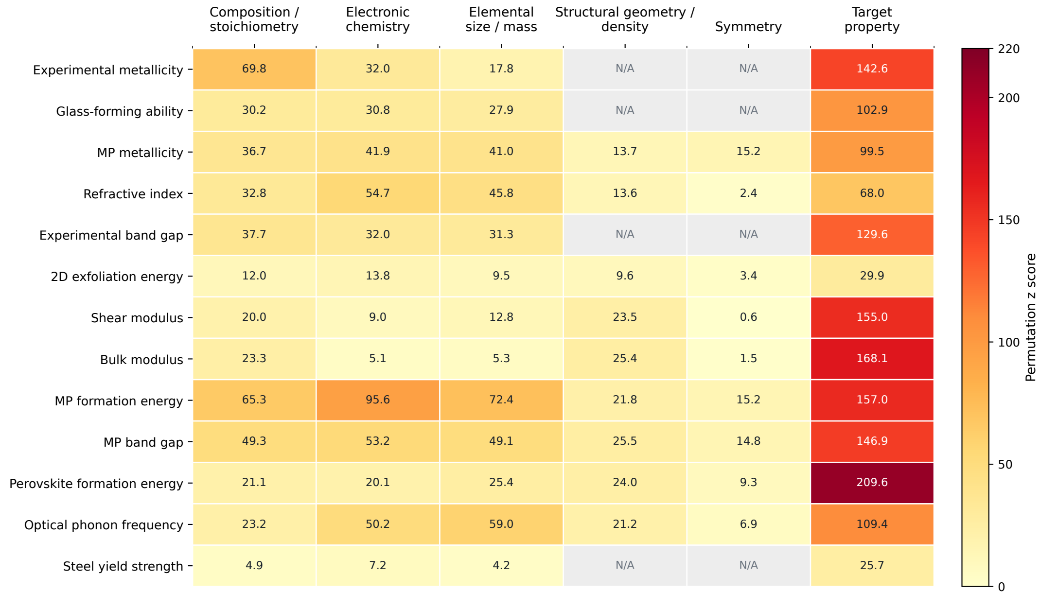
b Permutation z scores for representation-descriptor alignment
