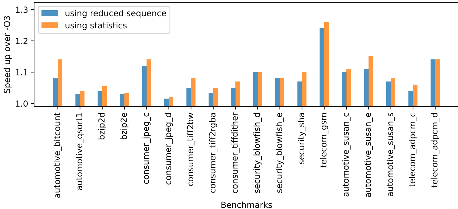
Comparison of Methods on cBench
