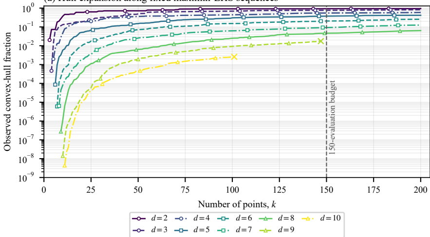
(a) Hull expansion along fixed maximin-LHS sequences
