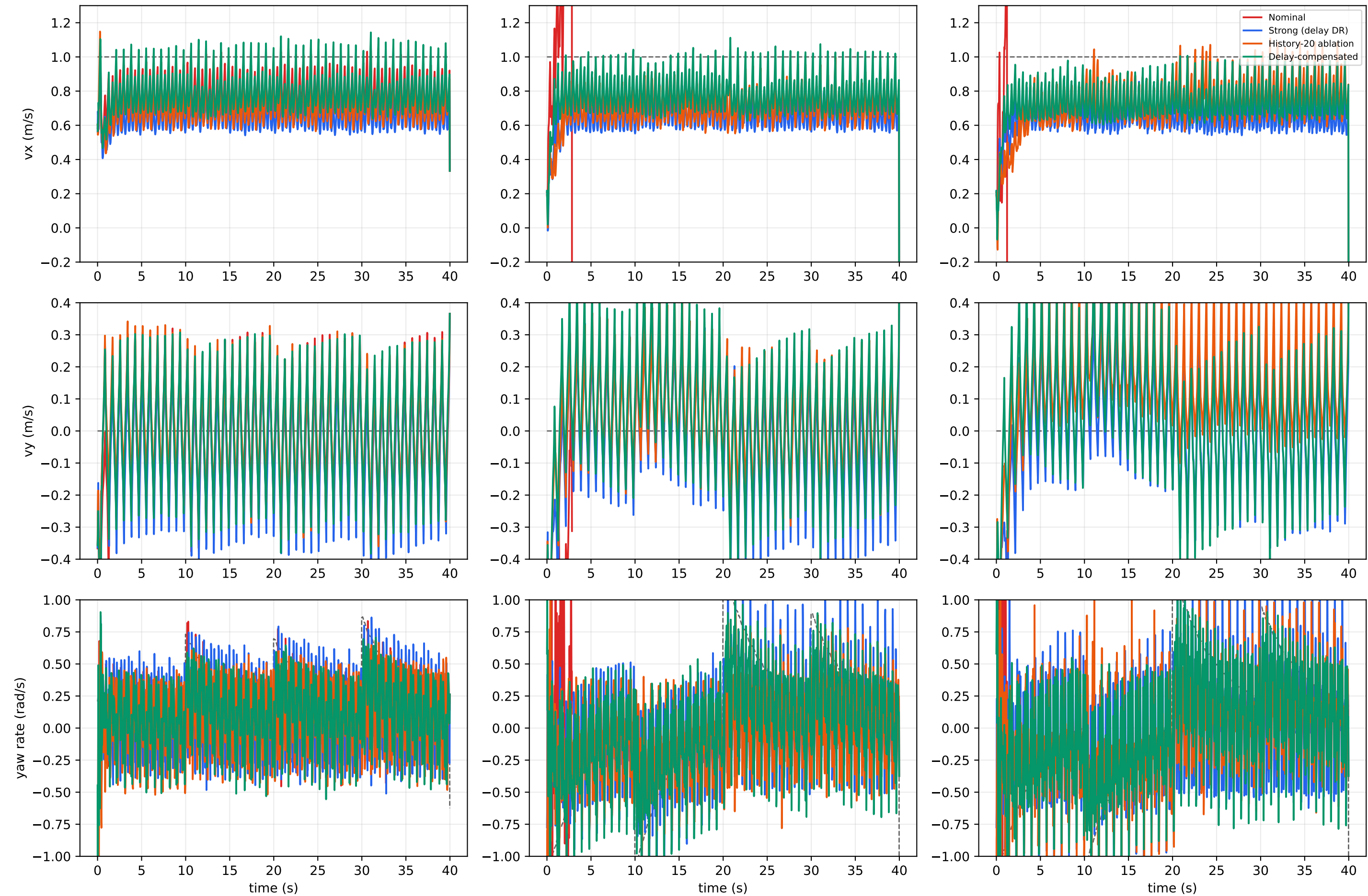
Velocity tracking time-series: vx, vy, yaw (lin_vel_x=1.0, lin_vel_y=0)
