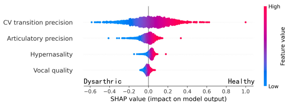
Fig. 3. The relationship between the interpretable layer's output and the SHAP values. Larger output values steer the model's decision toward "Healthy," which aligns with the clinical interpretations of the corresponding interpretable features.
