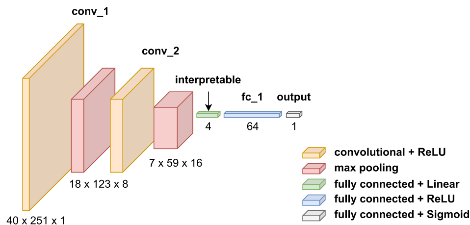
Fig. 1. The structure of the proposed DNN model. The 4-unit layer is placed between the convolutional layers and a larger fully connected layer to both learn the features characterizing different aspects of dysarthria and to function as a bottleneck feature extractor.
