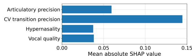
Fig. 2. The mean absolute SHAP values computed from the cross-validation ( w=0.7 ). CV transition precision has the largest SHAP value, suggesting the largest contribution to the classification.
