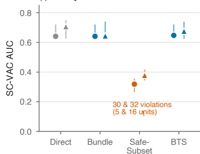
(f) Safety-constrained AUC
