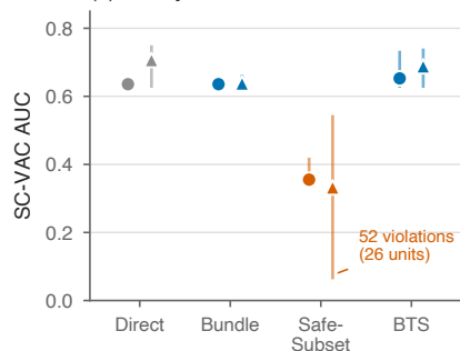
(c) Safety-constrained AUC
