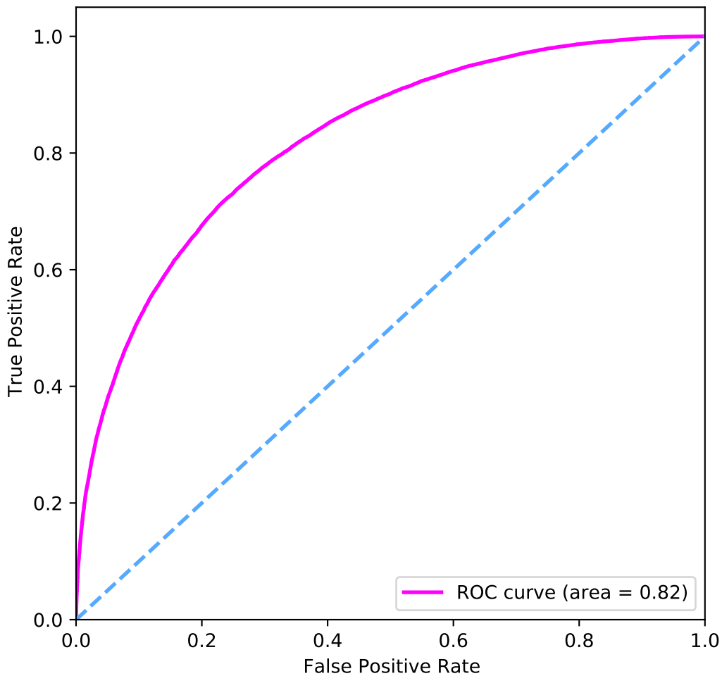
ROC DNN
