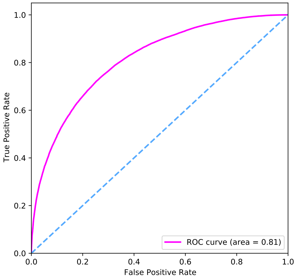
ROC Tensorflow
