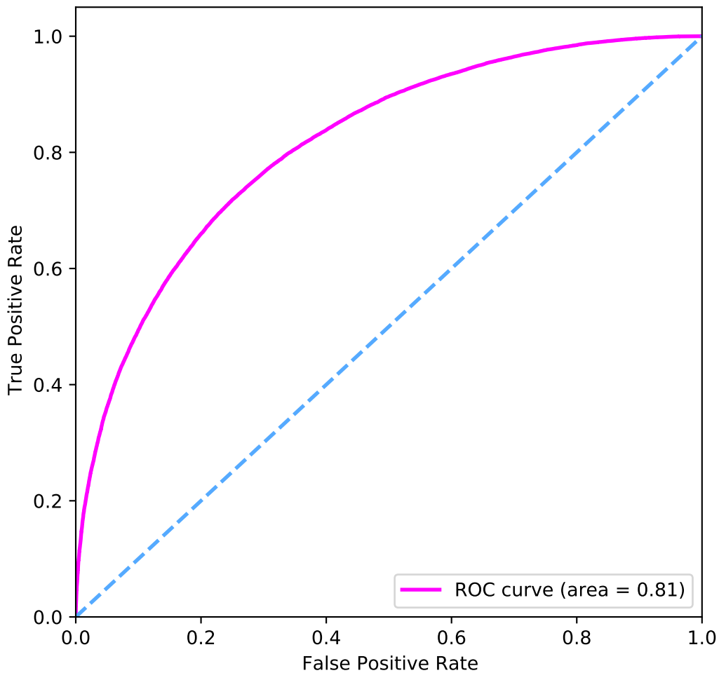
ROC Tensorflow
