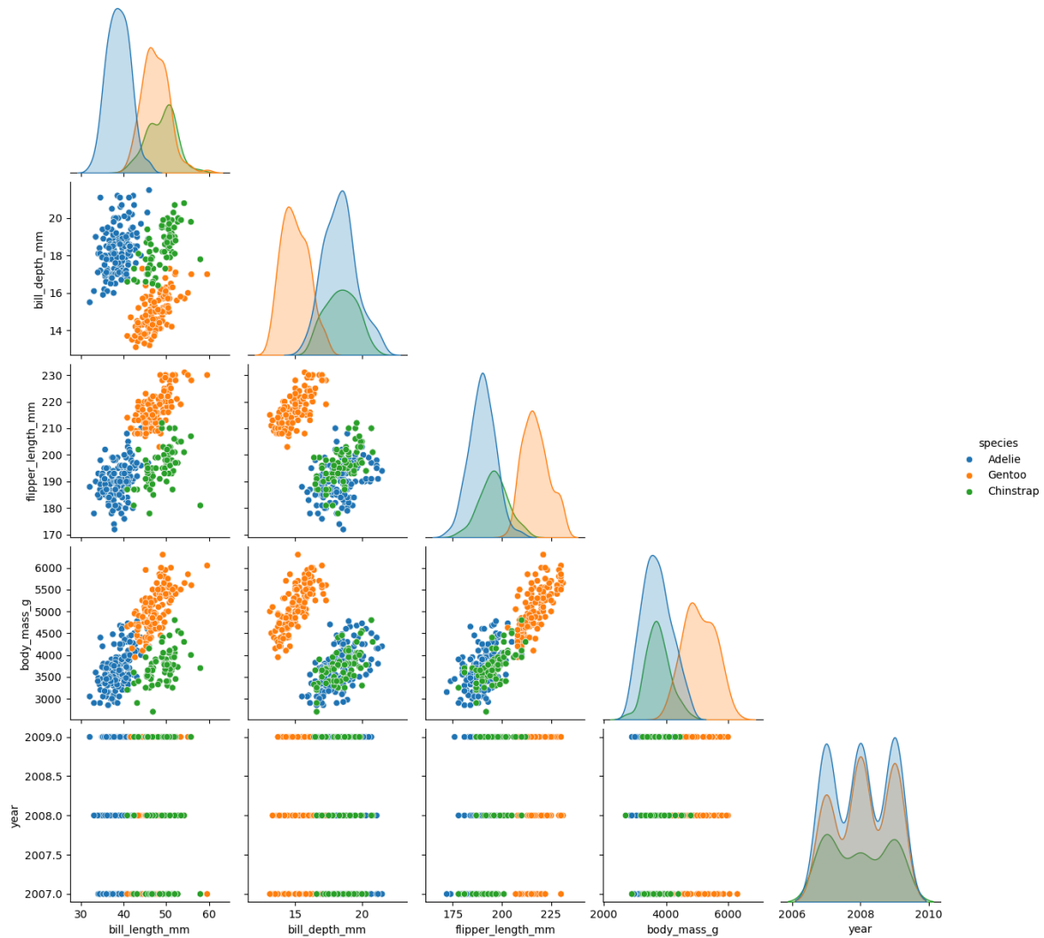
Pair plots of all numerical variables, colored by species. Colour by species and the clouds line up.
