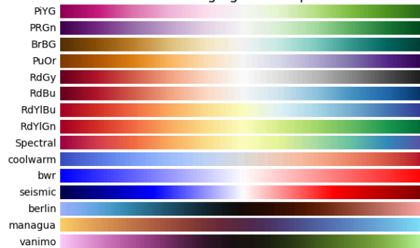
Diverging colormaps
