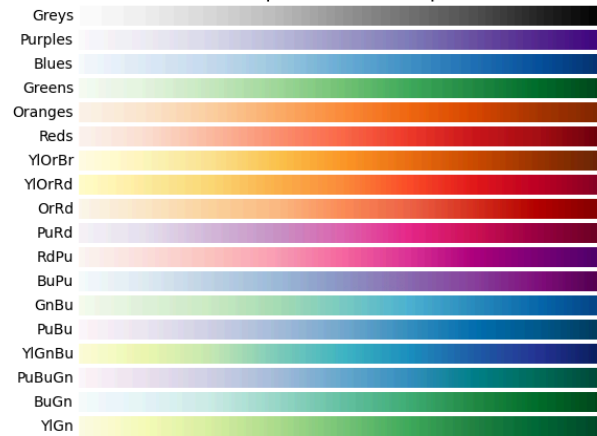
Sequential colormaps
