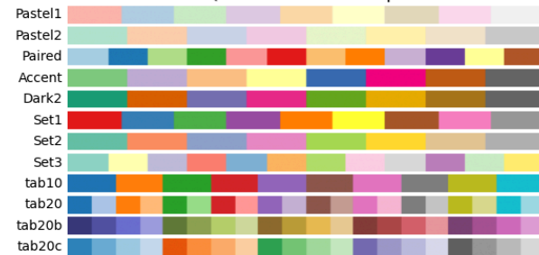
Qualitative colormaps
