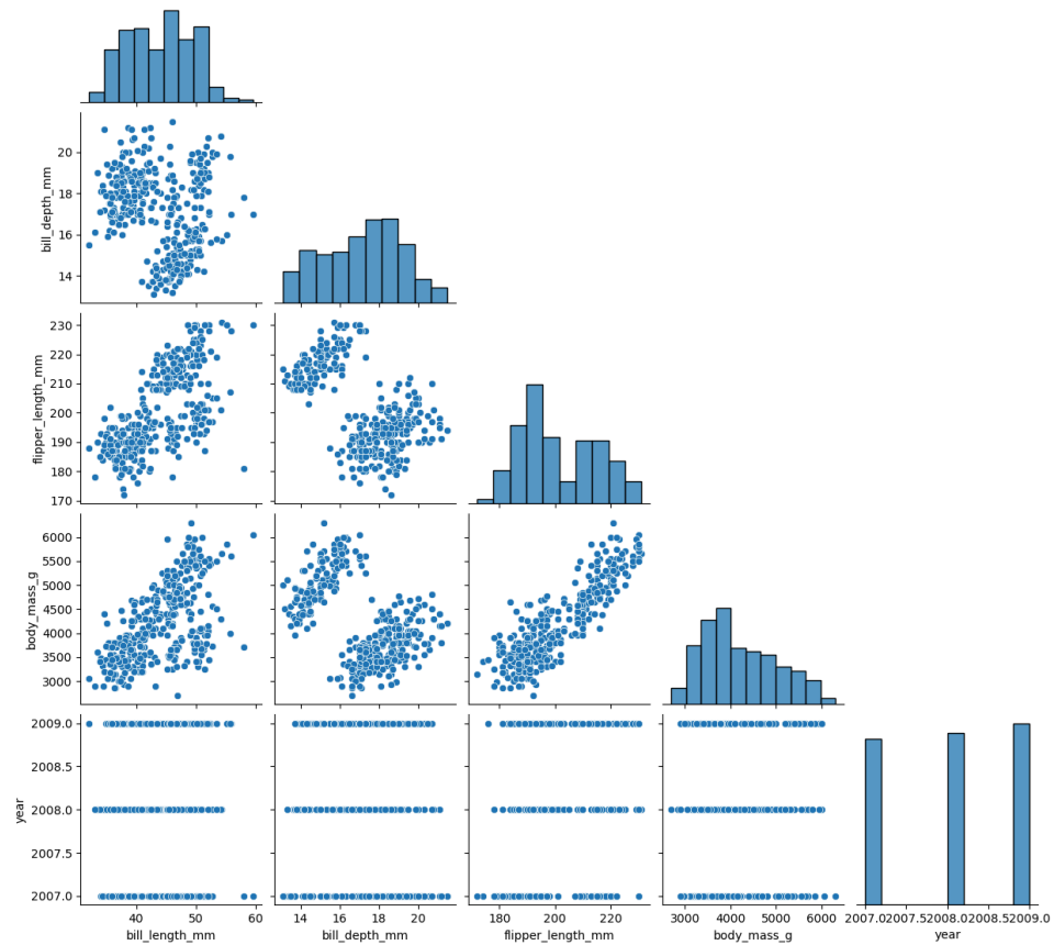
Pair plots of all numerical variables.
