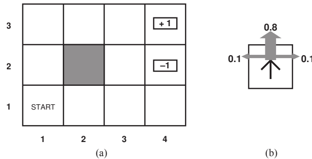
Figure 2. (a) A simple 4 \times 3 environment that presents the agent with a sequential decision problem. The two terminal states have reward +1 and -1, respectively, and all other states have a reward of -0.04. (b) Illustration of the transition model of the environment: the “intended” outcome occurs with probability 0.8, but with probability 0.2 the agent moves at right angles to the intended direction. A collision with a wall results in no movement.
