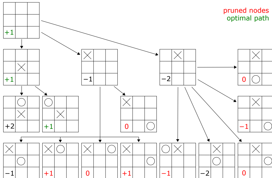
Figure 1. Nodes in red correspond to nodes that would have been pruned, i.e. not evaluated, if \alpha - \beta pruning was applied, assuming the nodes are generated in the optimal order for \alpha - \beta pruning.
