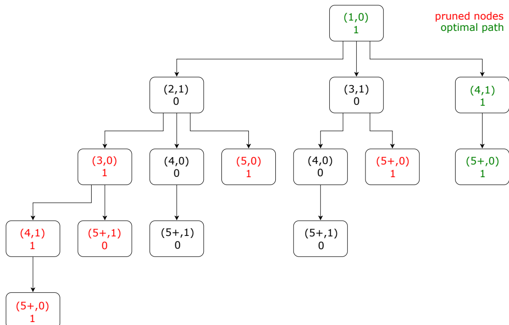
Figure 2. Nodes in red correspond to nodes that would have been pruned, i.e. not evaluated, if \alpha - \beta pruning was applied, assuming the nodes are generated in the optimal order for \alpha - \beta pruning.
