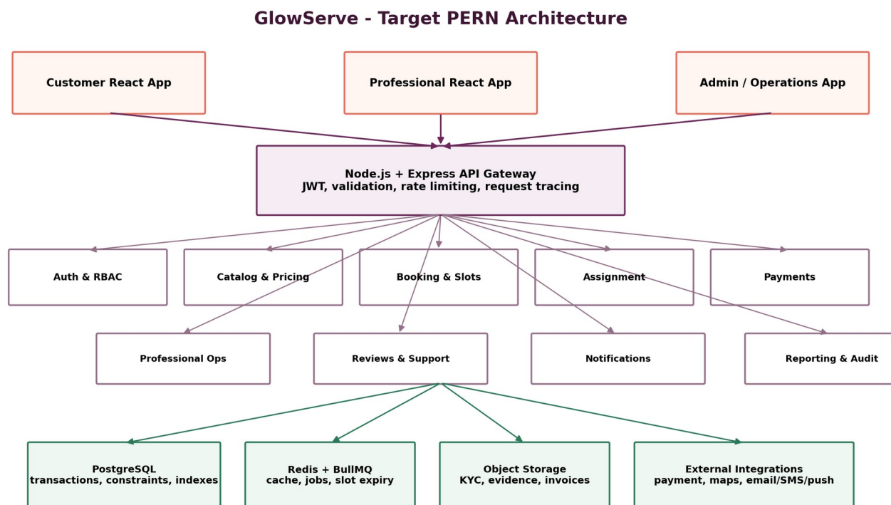
Figure 2. Target modular-monolith architecture and external dependencies.
